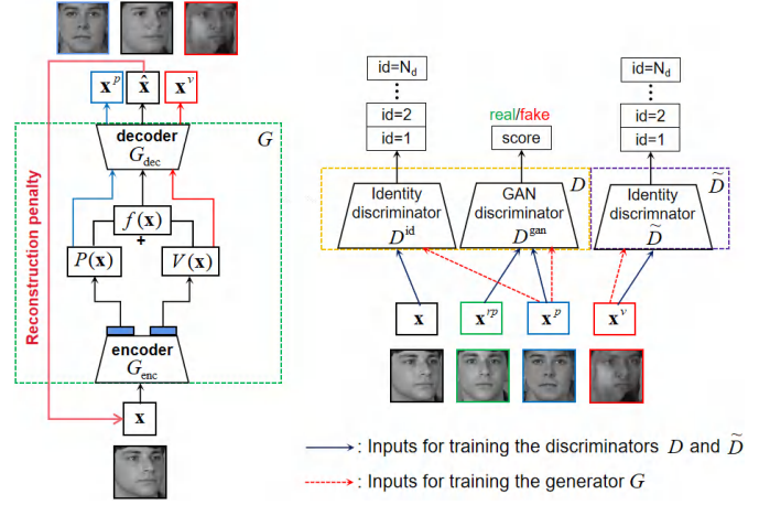
Fig. 2. Architecture of the proposed DisP+V. \mathbf{x} , \mathbf{x}^p , \mathbf{x}^v , \hat{\mathbf{x}} , and \mathbf{x}^{\text{rp}} are the input face, the generated prototype, the generated variation, the reconstructed face, and the real prototype, respectively. P(\mathbf{x}) and V(\mathbf{x}) are the disentangled prototype and variation features in the encoded latent space, respectively, and f(\mathbf{x}) = P(\mathbf{x}) + V(\mathbf{x}) . When training D , D^{\text{id}} predicts the identity label of \mathbf{x} , and D^{\text{gan}} assigns a high score to the real prototype \mathbf{x}^{\text{rp}} but a low score to the generated prototype \mathbf{x}^p . When training \tilde{D} , \tilde{D} predicts the identity of \mathbf{x}^v . When training G , the generated prototype \mathbf{x}^p aims to fool D^{\text{id}} and D^{\text{gan}} to classify it into the identity label of \mathbf{x} and to assign it a high score of being real prototype, respectively; the reconstructed face \hat{\mathbf{x}} aims to well reconstruct the input face \mathbf{x} ; and the generated variation \mathbf{x}^v aims to fool \tilde{D} to output a constant vector with a uniform distribution.
