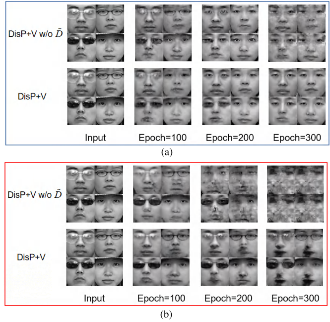
Fig. 7. Examples of generated prototypes and variations by DisP+V and DisP+V w/o \tilde{D} on CAS-PEAL dataset when the number of training epochs increases from 100 to 300. (a) Generated prototypes. (b) Generated variations.
