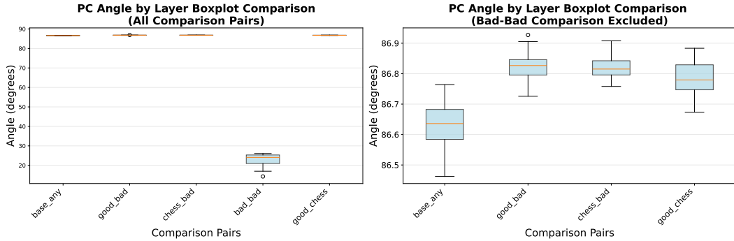
Figure 8: Principal angle measurements between parameter subspaces. The bad_bad comparison yields mean principal angles of approximately 20^{\circ} – 25^{\circ} , while all other comparison groups exhibit near-orthogonality.
