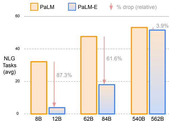
Figure 5: Results on general language tasks (NLG = natural language generation): increasing scale leads to less catastrophic forgetting between a corresponding PaLM-E model and its inherited PaLM model. See full suite of tasks and results in Tab. 10.
