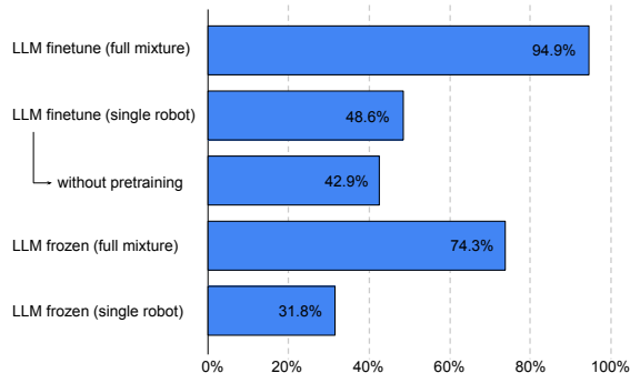
Figure 3: Planning success results in the TAMP environment (1% data) for PaLM-E-12B, comparing of the effects of PaLM-E models (i) using the full training mixture, (ii) pre-training (ViT and PaLM), and (iii) freezing or finetuning the language model. Transfer from full mixture is particularly effective. Note that full mixture contains only 1% of the training data (320 examples each) for the tasks evaluated here. Shown is the mean of tasks p_1 , p_2 .
