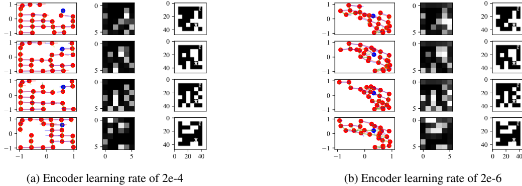
Figure 7: Ablation of the learning rates for the encoder, where a too low learning rate causes collapse of z^c and a too high learning rate causes distortions in the uncontrollable features z^u . In both figures, the left column is z^c \in \mathbb{R}^2 , the middle column is z^u \in \mathbb{R}^{6 \times 6} and the right column is the input state \in \mathbb{R}^{48 \times 48} .
