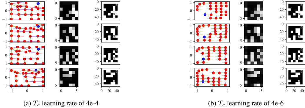
Figure 8: Ablation of the learning rates for the action-conditioned forward predictor. A too high learning rate will cause the controllable representation to lose structure, while a low learning rate retains structure but does not learn strong transition dynamics. In both figures, the left column is z^c \in \mathbb{R}^2 , the middle column is z^u \in \mathbb{R}^{6 \times 6} and the right column is the input state \in \mathbb{R}^{48 \times 48} .
