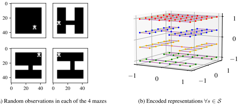
Figure 1: Visualization in a maze environment of (a) four random states \in \mathbb{R}^{48 \times 48} and (b) the disentanglement of the controllable latent z^c \in \mathbb{R}^2 on the horizontal axes, and the uncontrollable latent z^u \in \mathbb{R}^1 on the vertical axis, given for all states in the four maze environments shown in four different colors. The representation is trained on high-dimensional tuples (s_t, a_t, r_t, s_{t+1}) , sampled from a replay buffer \mathcal{B} , gathered from random trajectories in the four maze environments shown in (a). All possible states are encoded with z_t = f(s_t; \theta_{enc}) and plotted in (b) with the transition prediction for each possible action, revealing a clear disentanglement between the controllable agent’s position and the uncontrollable wall architecture. Note that all samples are taken from the same buffer, filled with samples from all four mazes.
