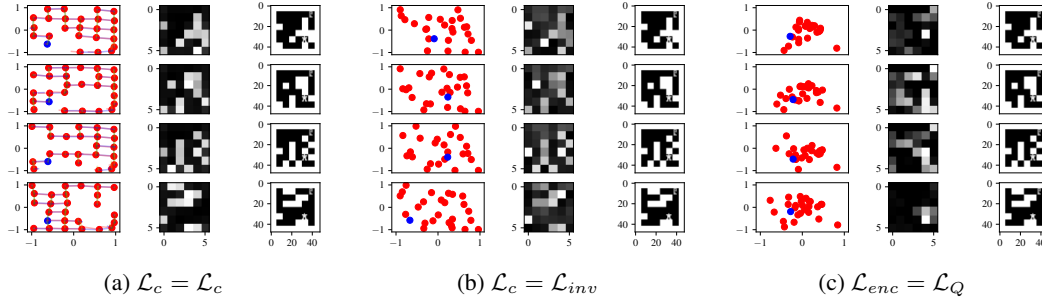
Figure 3: A plot of the latent representation for all observations in a single randomly sampled maze when training with either the aforementioned losses (a), substitution of the action-conditioned forward-prediction loss \mathcal{L}_c for an inverse-prediction loss \mathcal{L}_{inv} (b) and end-to-end updating the encoder with only the Q-loss \mathcal{L}_Q from DDQN for 500k iterations (c). In all three settings, the left column shows the controllable latent z_t^c \in \mathbb{R}^2 with the current state in blue, the other possible states in red, and the predicted movement due to actions as different colored bars for each individual action. The middle column shows the uncontrollable latent z_t^u \in \mathbb{R}^{6 \times 6} and the right column shows the original state s_t \in \mathbb{R}^{48 \times 48} . Evidently, the controllable representations in (b) and (c) lack disentanglement and interpretability. Furthermore, the representation in (c) seems to have very little structure at all, showing that a representation that is optimized without prior structural incentives will often represent a black box.
