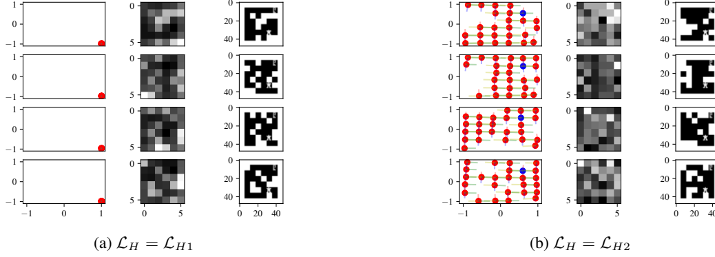
Figure 10: In both figures, the left column is z^c \in \mathbb{R}^2 , the middle column is z^u \in \mathbb{R}^{6 \times 6} and the right column is the input state \in \mathbb{R}^{48 \times 48} .
