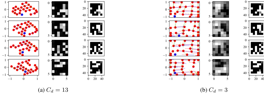
Figure 6: Ablation of the hyperparameter C_d , where a higher value of C_d enforces less entropy in the representation, while a lower value of C_d especially pushes the controllable features z^c towards shapes that ensure large distances between samples. In both figures, the left column is z^c \in \mathbb{R}^2 , the middle column is z^u \in \mathbb{R}^{6 \times 6} and the right column is the input state \in \mathbb{R}^{48 \times 48} .
