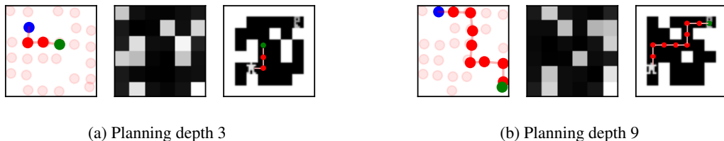
Figure 5: Visualization of the latent representation through an actual planning iteration utilizing a planning depth of 3 (a) and a planning depth of 9 (b), with the controllable representation z^c \in \mathbb{R}^2 (left), the uncontrollable representation z^u \in \mathbb{R}^{6 \times 6} (middle) that is kept static throughout planning depth and the original pixel input s_t \in \mathbb{R}^{48 \times 48} (right). The translucent red dots represent every possible encoded state in the random maze environment, the full blue dot represents the current encoded state, the red dots represent intermediate encoded states estimated by planning and the green dot represents the final predicted state as chosen by the planning algorithm, consistent with its depth.
