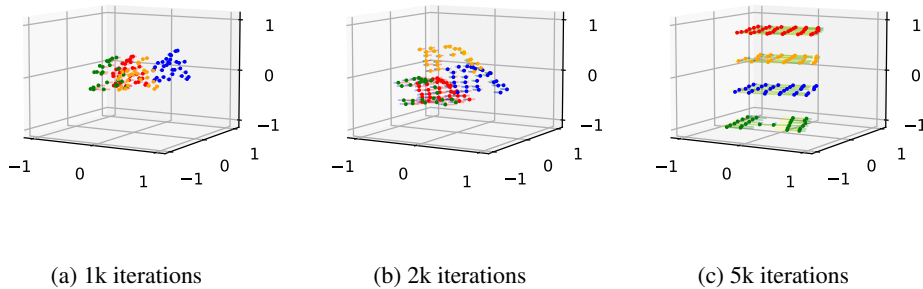
Figure 13: Progression of the separation of the controllable z^c (x and y-axis) and uncontrollable z^u (z-axis) features in the maze environment.
