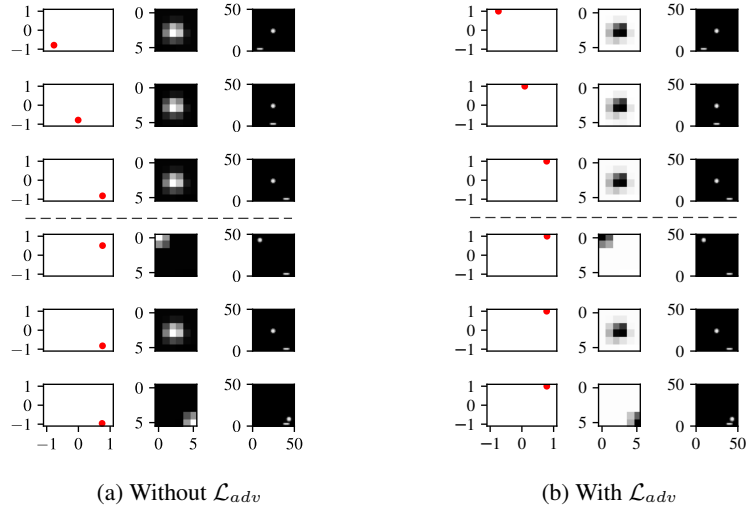
Figure 14: Visualization of the latent feature disentanglement in the catcher environment after 200k training iterations, with z_t = f(s_t; \theta_{enc}) \in \mathbb{R}^2 + \mathbb{R}^{6 \times 6} . In (a) and (b), the left column shows z_t^c , the middle column is a feature map representing z_t^u and the right column is the pixel state s_t . The dashed lines separate observations where the ball position or the paddle position is kept fixed for illustration purposes. z^c tracks the agent position while z^u tracks the falling ball. In b), note that even when having a two-dimensional controllable state (only 1 is needed, see Appendix D.2), the adversarial loss makes sure that distinct ball positions have a negligible effect on z^c , even when the high-level features of the agent and the ball might be hard to distinguish.
