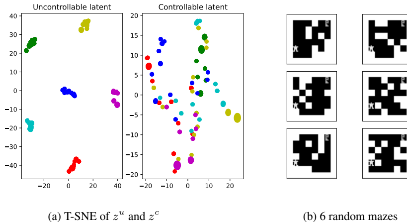
Figure 12: Ablation of a dimensionality increase in our random maze environment. Here, the total latent space is a 32-dimensional MLP output, where z^c and z^u are both 16-dimensional. in (a), 6 random trajectories are plotted using T-SNE (perplexity=20) in different colors for both z^c and z^u , where z^u remains similar across a trajectory (same wall architecture), and z^c differs across the trajectory (different agent positions). In (b), a collection of the random mazes are shown from which the random trajectories have been taken.
