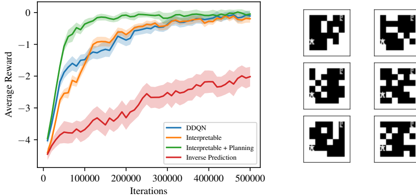
Figure 4: Performance of different (pre)trained representations on the random maze environment, measured as a mean (full line) and standard error (shaded area) over 5 seeds. The ‘Interpretable’ setting uses an encoder pre-trained with 50k iterations to acquire a representation as in Fig. 3a, after which the encoder is frozen and a Q-network is trained on top with DDQN for 500k iterations. The ‘Interpretable + Planning’ curve is similar to the ‘Interpretable’ setting but uses DDQN with a planning algorithm in the controllable partition of the latent space with a depth of 3. The ‘DDQN’ setting uses an encoder trained end-to-end with only DDQN for 500k iterations and the ‘Inverse Prediction’ setting is equal to the ‘Interpretable’ setting but has an encoder pre-trained with \mathcal{L}_{inv} instead of \mathcal{L}_c . On the right, a random subset of the vast amount of procedurally generated mazes used in the reward evaluation is shown.
