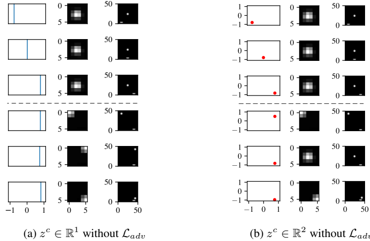
Figure 15: Comparison of training the representation for the catcher environment with either 1 or 2-dimensions for the controllable representation z^c . When using more dimensions for z^c than needed, it can be observed that some information of the ball position can be present in z^c .
