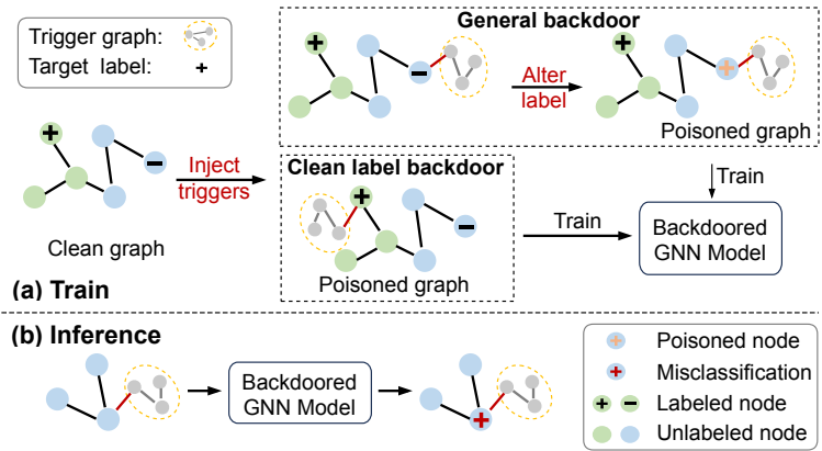
Figure 1: Illustration of graph backdoor attacks under both the general and clean-label settings.
