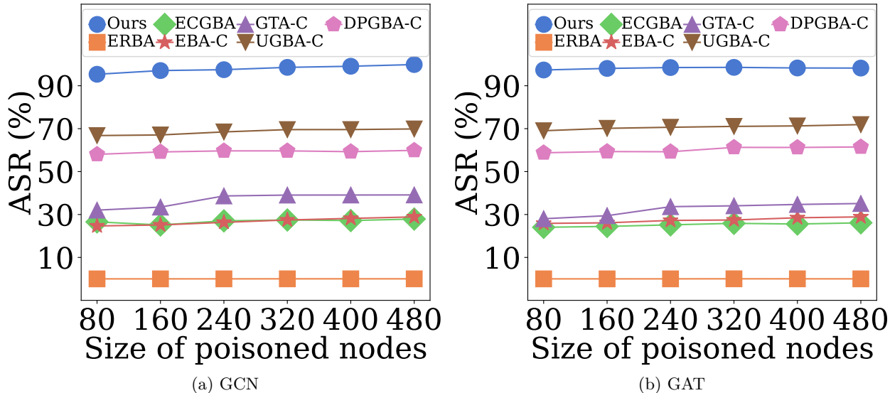
Figure 10: Impact of attack budget.
