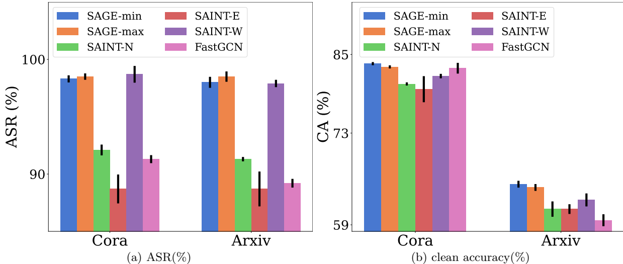
Figure 6: Performance of BA-LOGIC on sampling-based GNNs.
