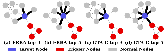
Figure 2: GNNExplainer’s visualization of important subgraphs in a poisoned node’s computational graph. We bold the edges connecting the poisoned node and the top-3 (a, c) and top-5 (b, d) most important nodes, respectively.
