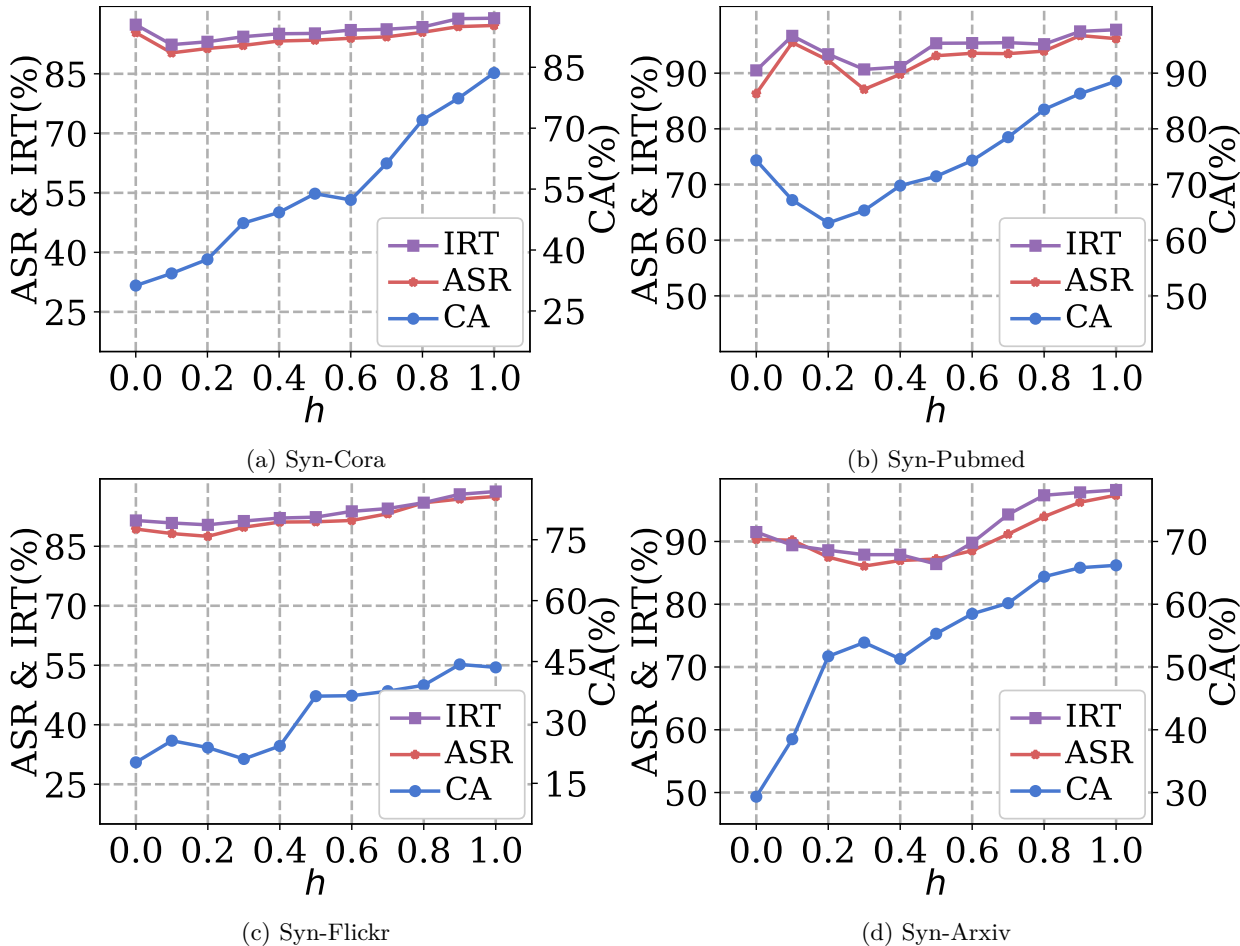
Figure 11: Performance of BA-LOGIC on synthetic graphs with different feature-label correlations.
