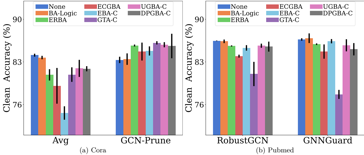
Figure 7: Clean accuracy of backdoored models.
