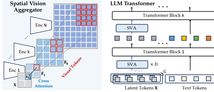
Figure 7: Spatial Vision Aggregator (SVA) . We propose SVA, a dynamic and spatially-aware connector that integrates multiple vision features with LLMs while reducing the number of tokens. 9
