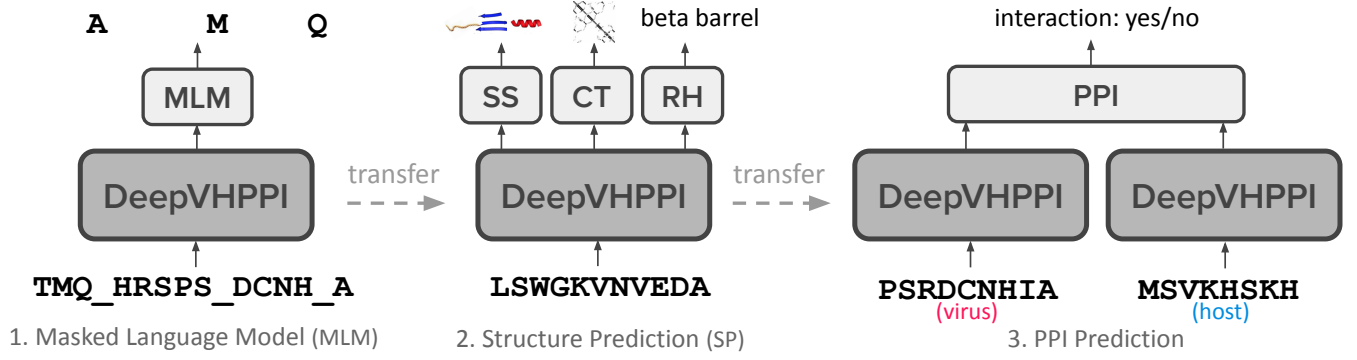
Figure 3: Transfer Learning Framework for DeepVHPPI. First, we pretrain the network on the Masked Language Model (MLM) task from a large repository of unlabeled protein sequences. Second, we further pretrain the network on a set of Structure Prediction (SP) tasks including secondary structure (SS), contact (CT), and remote homology (RH). Finally, we fine-tune the network on the protein-protein interaction (PPI) prediction task. The base DeepVHPPI shown as the large dark grey block is shared across all tasks, and each task uses its own classifier, shown as small light grey blocks.
