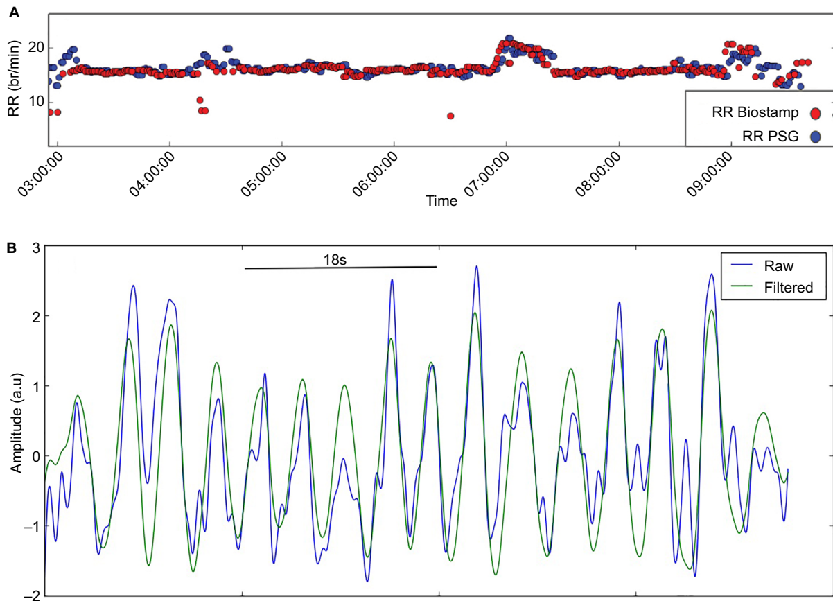
Figure 1 Respiration measurements. Notes: (A) Overlaid calculations of respiratory rate (RR) from the BiostampRC® system (red dots) and the PSG recording (blue dots) for a full night of recording in the lab. (B) Overlaid raw (blue) and filtered (green) signal of respiration from the BiostampRC®.
