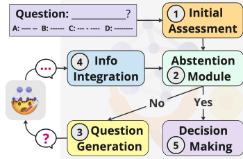
Figure 3: Expert system information flow breakdown.
