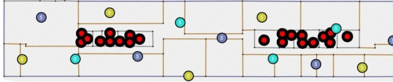
Fig. 1. Optimized network with indication of locations of the APs on the grand plan (90 m × 17 m) and their EIRP (inside dot). Different non-overlapping channels of Wi-Fi are indicated with different colors (channel 1= dark blue, channel 6 = light blue, channel 11 = green). Red flags mark rooms that do not require coverage.
