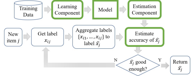
Figure 1: General online crowdsourcing process, in which the components with green solid frame are this work’s focus.
