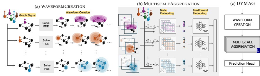
Figure 2: Visual illustration of DYMAG (a) Waveform bank creation solving PDEs. (b) Multiscale Aggregation by taking inner product with the waveforms. (c) DYMAG consists of stacked layers and a prediction head.
