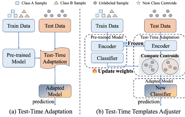
Fig. 2: The Idea of Test-time Adaptation.
