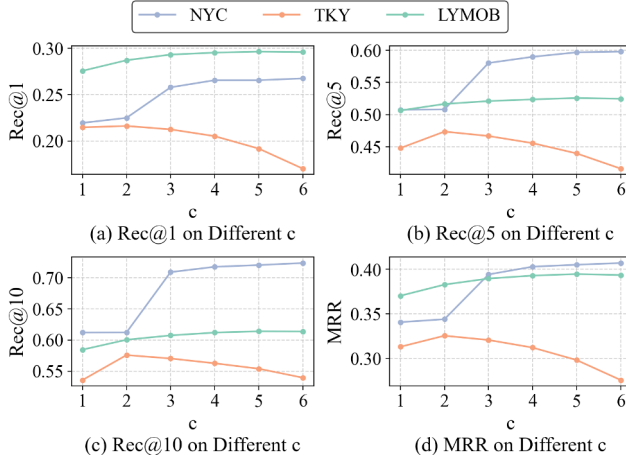
Fig. 6: Impact of the Number of Sessions c .
