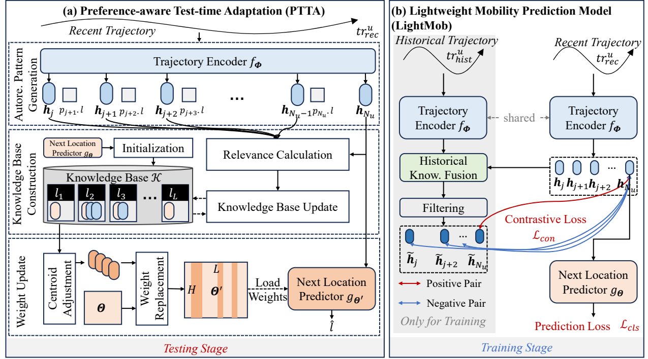
Fig. 3: Framework of AdaMove.
