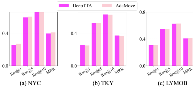
Fig. 9: AdaMove vs DeepTTA on Different Datasets.
