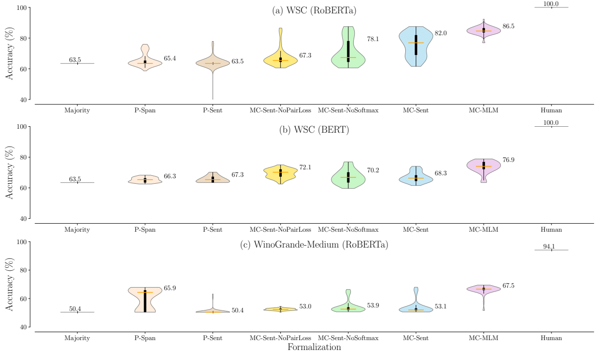
Figure 1: Plots of validation accuracy from 60 runs on each corpus. The orange line marks the median number and label marks 75 th percentiles.
