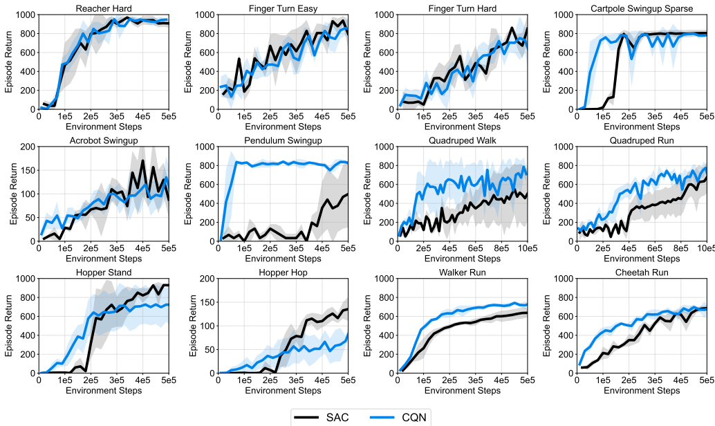
Figure 10: State-based DMC results. Learning curves on 12 state-based robotic locomotion tasks from DeepMind Control Suite [28], measured by the episode return. The solid line and shaded regions represent the mean and confidence intervals, respectively, across 4 runs.
