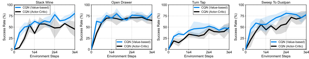
Figure 7: Simulation results on 20 sparsely-rewarded tasks from RL Bench [1]. All experiments are initialized with 100 expert demonstrations and all RL methods have an auxiliary BC objective. We report the success rate over 25 episodes. The solid line and shaded regions represent the mean and confidence intervals, respectively, across 3 runs.
