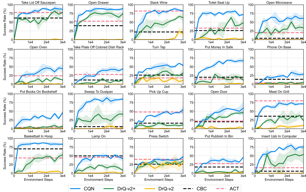
Figure 4: Simulation results on 20 sparsely-rewarded tasks from RL Bench [1]. All experiments are initialized with 100 expert demonstrations and all RL methods have an auxiliary BC objective. We report the success rate over 25 episodes. The solid line and shaded regions represent the mean and confidence intervals, respectively, across 3 runs.
