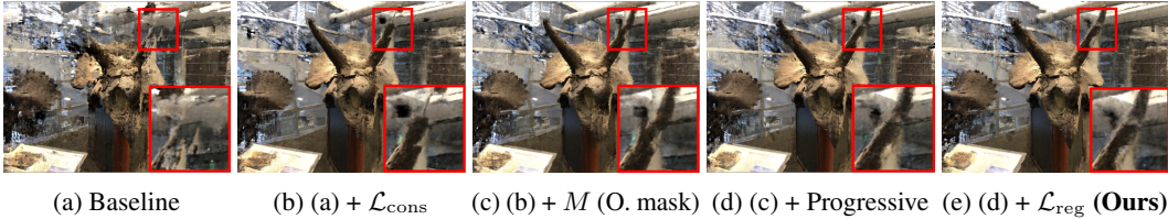
Figure 7: Qualitative ablation. Our qualitative ablation results on Horns scene shows the contribution of each module in performance of our model at 3-view scenario.
