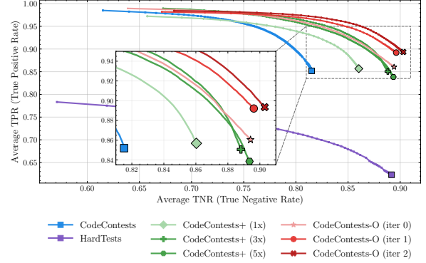
Figure 1: Pareto frontiers of TPR (True Positive Rate, proportion of correct solutions accepted, measuring test case fidelity) and TNR (True Negative Rate, proportion of incorrect solutions rejected, measuring discriminability) across different datasets. Our CodeContests-O consistently outperforms prior datasets, demonstrating superior test case quality. The iterative refinement process (iter 0-2) progressively enhances both metrics, validating the effectiveness of our feedback-driven approach.
