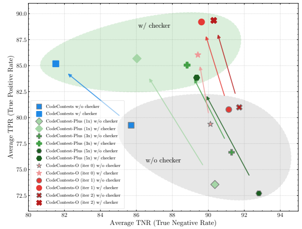
Figure 3: Effect of logic-based checker on TPR and TNR. "w/o checker" denotes string-matching evaluation, while "w/ checker" employs the logic-based checker. The checker consistently improves TPR across all datasets by correctly validating solutions with multiple valid outputs. CodeContests-O with checker achieves the optimal balance, demonstrating the effectiveness of our synchronized checker generation strategy.
