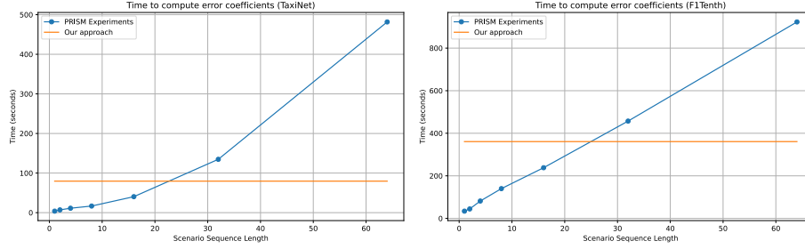
Fig. 6: Time needed to construct the error coefficients vector \mathbf{b} using our compositional approach vs. a non-compositional application of PRISM’s Experiments feature. For our approach, we report the time needed for the one-time summary generation, which can then be composed with minimal overhead for any sequence of scenarios. For PRISM experiments, we report the time needed to compute \mathbf{b} for fixed scenario sequences of varying length. For TaxiNet we chose scenario sequences containing only bright , for F1Tenth we chose scenario sequences containing only right .
