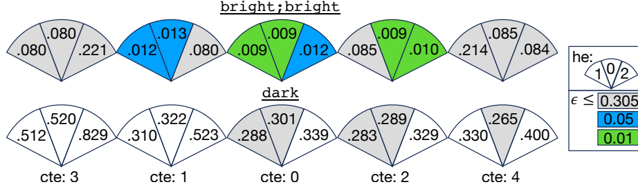
Fig. 5: Error probability by initial point distribution for bright;bright and dark scenarios. Initial point distributions that ensure error probability at most 0.305, 0.05 and 0.01 are highlighted in gray, blue, and green, respectively.
