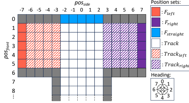
Fig. 4: Each F1Tenth scenario corresponds to a track segment.
