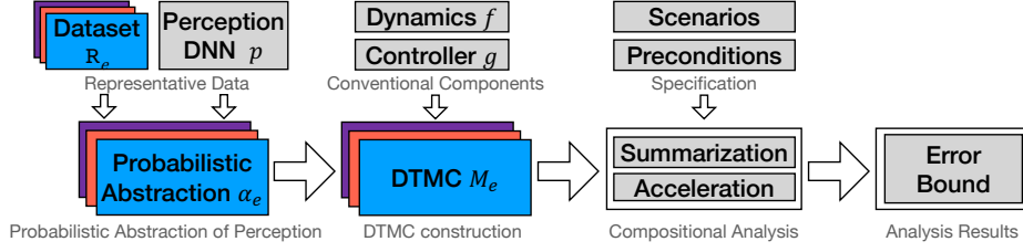
Fig. 3: Scenario-based compositional analysis of autonomous systems.
