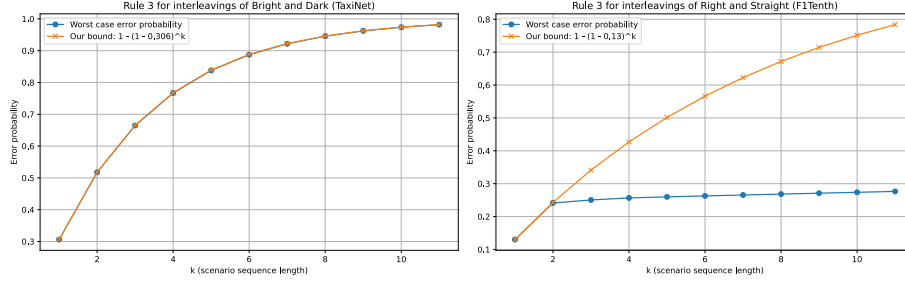
Fig. 7: The error bounds found by applications of Rule 3 vs. true worst-case error probability. For the worst case error probabilities, we consider all possible scenario interleavings and all starting distributions that satisfy the precondition \phi_\epsilon used in our application of Rule 3.
