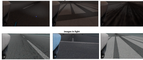
Fig. 2: TaxiNet achieves 91.25% accuracy when estimating heading for a bright image dataset but only 53.87% accuracy for a dark image dataset.
