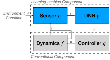
Fig. 1: Components of an autonomous system with DNN-based perception.
