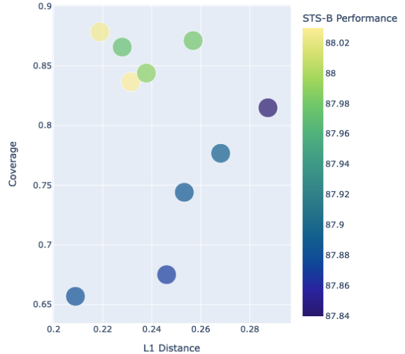
Figure 4: Performance of HyperLoRA trained on different source dialects with respect to L1 distance and Coverage metric
