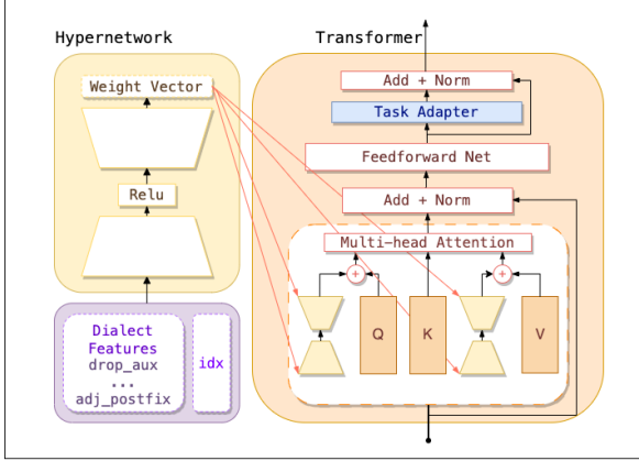
Figure 1: HyperLoRA Architecture. During training, only hypernetwork weights are updated and there is no task adapter in the main model. At inference, the task adapter and its classification head are added.
