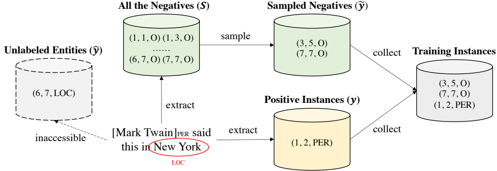
Figure 1: An example to depict how negative sampling collects training negatives given an annotated sentence. The phrase marked by a red circle is an unlabeled entity.
