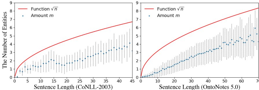
Figure 2: The comparisons between changes of entity number and square root curve.
