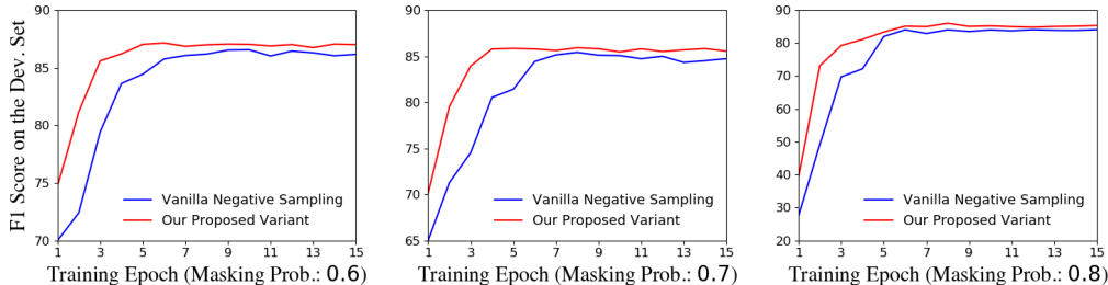
Figure 3: The changes of F1 scores with training epochs on some synthetic datasets.
