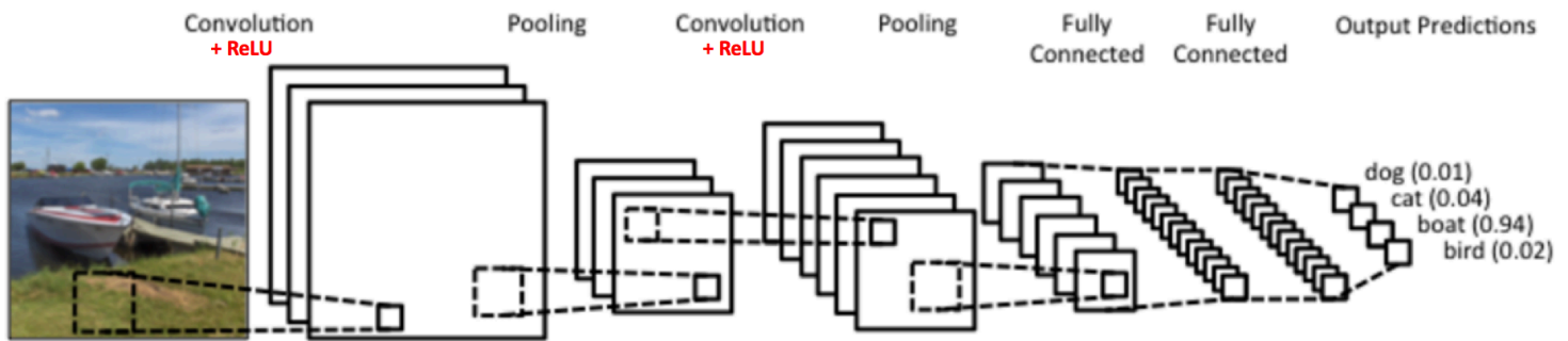
Figure 3: A simple ConvNet. Source [5( https://www.clarifai.com/technology/ )]
