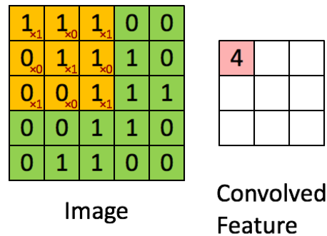
Figure 5: The Convolution operation. The output matrix is called Convolved Feature or Feature Map.
