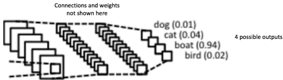
Figure 14: Fully Connected Layer -each node is connected to every other node in the adjacent layer Apart from classification, adding a fully-connected layer is also a (usually) cheap way of learning non-linear combinations of these features. Most of the features from convolutional and pooling layers may be good for the classification task, but combinations of those features might be even better [11 ( https://stats.stackexchange.com/questions/182102/what-do-the-fully-connected-layers-do-in-cnns/182122#182122 )].
