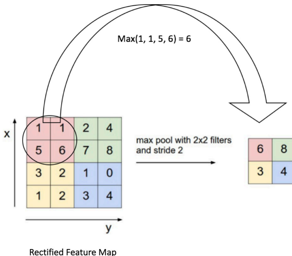
Figure 10: Max Pooling. Source [4 ( http://cs231n.github.io/convolutional-networks/ )]
