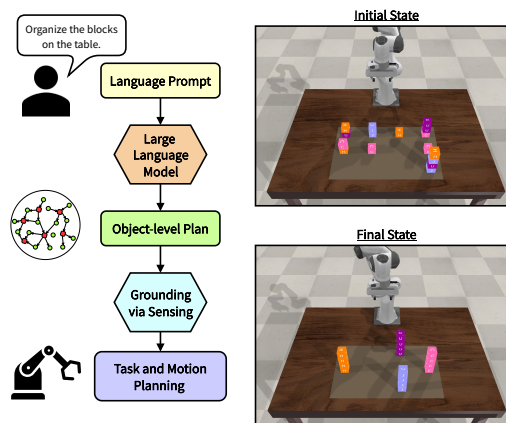
Figure 1: Our approach prompts an LLM for object-level information with which we construct an object-level plan (as FOON). This plan schema bootstraps task- and motion-level planning (TAMP) via PDDL subgoals.
