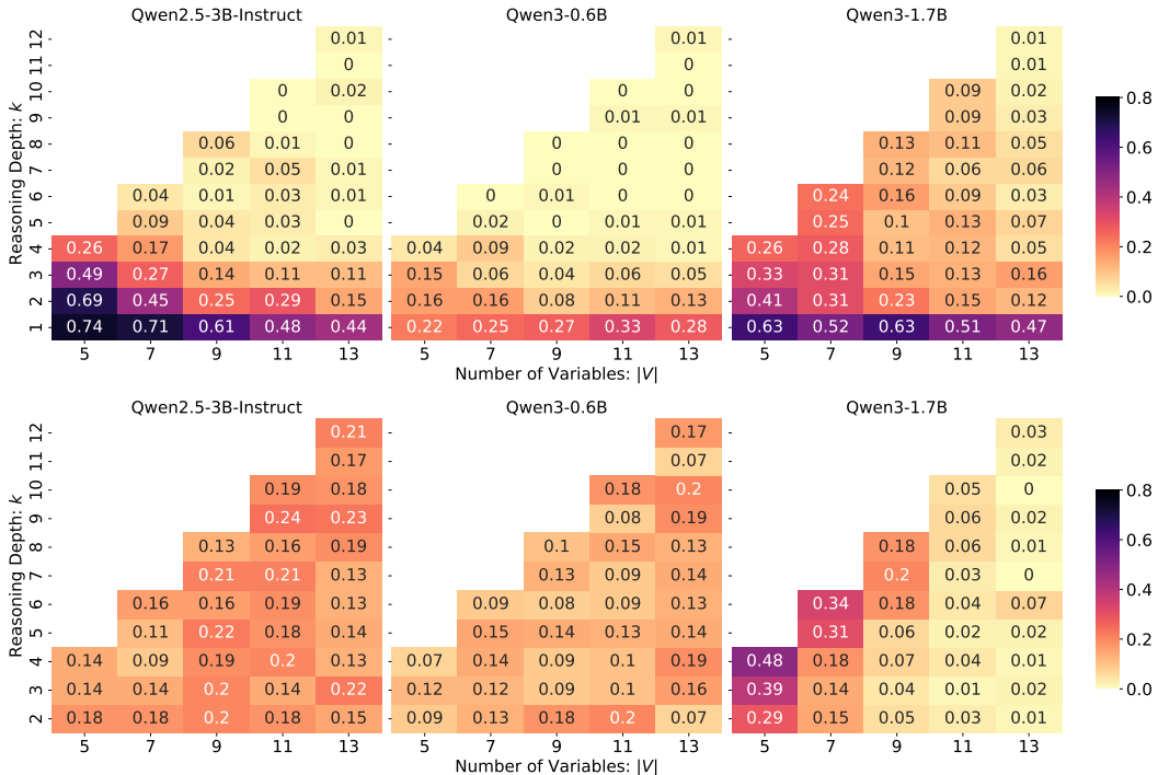
Figure 1: Performance of models on (a) answerable (top row) and (b) unanswerable (bottom row) instances in GRAPHLA, as a function of reasoning depth k and number of variables |V| .
