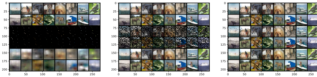
Figure 31: Image Completion Results using CNN Augmented MoE-NPs.
