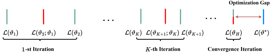
Figure 21: Illustration of Expectation Maximization for NPs. Green lines indicate the results after the E-steps while the red lines are for the M-steps in Algorithm (8). In the convergence iteration, the performance gap \mathcal{L}(\vartheta_H) - \mathcal{L}(\vartheta_{H-1}) is close to zero and the algorithm results in at least a local optimal solution. Values of these quantities are increased from the left to the right.
