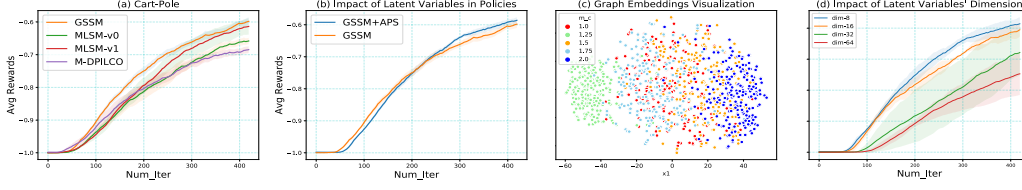
Figure 17: Experimental Results on Cart-Pole Tasks. (a) Learning curves of MBMRL algorithms using non-latent variable conditioned policies. (b) Learning curves of GSSM using (non-)latent variable conditioned policies. (c) t-SNE visualizations of latent variables in GSSM (samples are from 5 tasks with a pole mass as 1.0 and cart masses as \{1.0, 1.25, 1.5, 1.75, 2.0\} ). (d) Learning curves of GSSM+APS with different dimensions of latent variables. For all learning curves, the averaged rewards are tested after each iter in an offline way, and results indicate means and a standard error of the mean in 5 runs.
