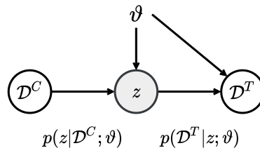
Figure 20: Deep Directed Latent Variable Models for Neural Processes. Here z is a global latent variable to summarize function properties. The model involves a functional prior distribution p(z|\mathcal{D}^C; \vartheta) and a functional generative distribution p(\mathcal{D}^T|z; \vartheta) . Please refer to Section (6.3) for the meaning of notations.
