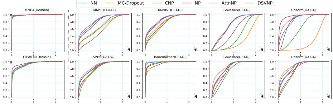
Figure 5: Cumulative Distribution Functions of Entropies in O.O.D. Detection Tasks. Values on X-axis are example entropies ranging from 0 to 2.3, and the y-axis records cumulative probabilities. The first row corresponds to the predictive result with models trained on MNIST, while the second is with models trained on CIFAR10. NN means the baseline neural network without a dropout layer. Curves in CDFs closer to triangular arrows reveal better uncertainty quantification.
