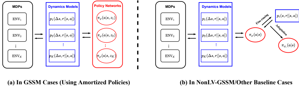
Figure 38: Meta Model-based Policy Search used in Models. Note that reducing adaptation time in policies is the first priority in this work. On the Left , amortized policies are used and latent variables are to specify different tasks. On the Right , the meta-trained policy is not conditioned on latent variables and needs to be adapted to respective tasks, which consumes additional time.
