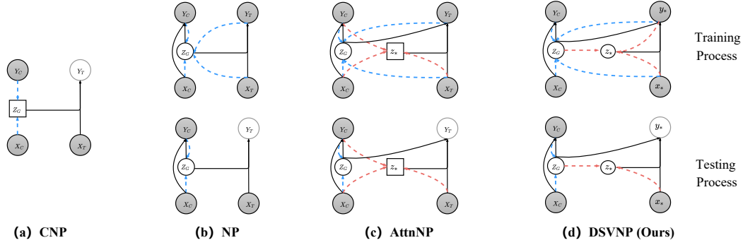
Figure 2: Probabilistic Graphs for CNP, vanilla NP, Attentive NP and DSVNP. The blue dotted lines characterize the inference towards global latent variable z_G , while the pink dotted lines are for target specific local latent variables z_* . The ones in the first row are training cases, while those in the second row are testing cases.
