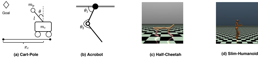
Figure 37: Fundamental Environments used in Meta Model-based Reinforcement Learning Experiments.
