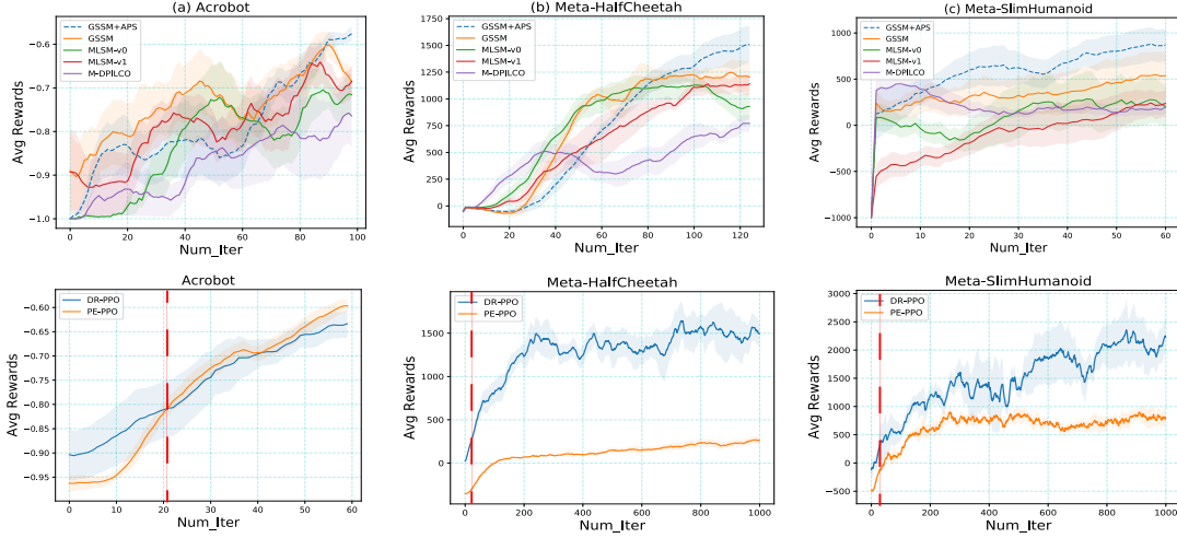
Figure 19: Performance of Policies in Meta-Training Processes. Figures in the first row are MBMRL results, while those in the second row are MFRL results (Red vertical dotted lines indicate the threshold of required time-steps used to train MBMRL baselines.). Here environments are varied in terms of dynamics during iterations. The average rewards are tested after each iter in an offline way, and results indicate means and corresponding standard errors of the mean in 5 runs.
