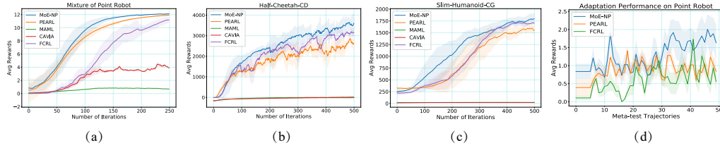
Figure 13: Results in Meta Learning Continuous Control. In (a)/(b)/(c): Learning curves show tested average returns with variances in 4 runs. 100 transitions are randomly collected from a task-specific memory buffer for point robot environments to infer the posterior. For Mujoco environments, 400 transitions are randomly collected from a task-specific memory buffer to infer the posterior. In (d): Fast Adaptation Performance in Meta Testing Point Robot Environments. The collected episodes are gradually increased to 50, and the average returns together with variances are visualized. 5 goals are sampled from the white part of arcs in Fig. (12.a).
