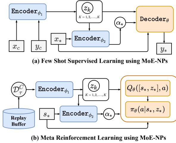
Figure 7: Computational Diagram of MoE-NPs in Meta Testing. In (a): The context variables are \mathcal{D}_\tau^C = [x_C, y_C] , and the expert latent variables z_{1:K} are approximated with neural networks. For discrete assignment latent variables e_* , we learn parameters of categorical distributions \alpha_* with neural networks. In (b): The context variables \mathcal{D}_\tau^C are sampled transitions from a memory buffer. During policy search, the selected expert latent variable z_* is a context variable in both Actor and Critic networks.
