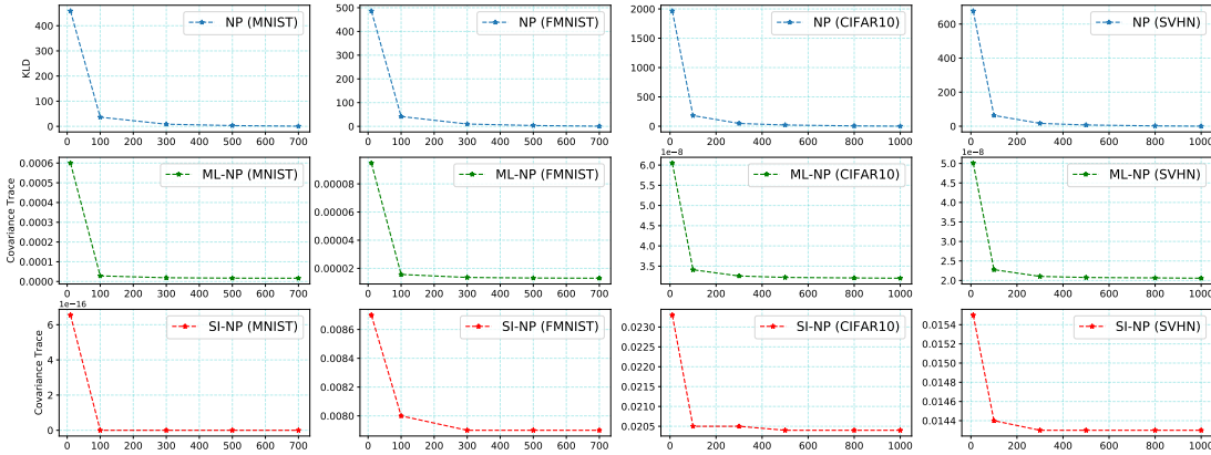
Figure 24: Statistics of Learned Functional Priors. In meta testing, we still vary the number of context points in image datasets. For NPs, the KL divergence value D_{KL}[q_\phi(z) \parallel q_\phi(z|\mathcal{D}_\tau^C)] is computed. For ML-NPs/SI-NPs, the trace of learned functional priors' covariance matrices \text{Tr}[\Sigma_\theta(\mathcal{D}_\tau^C)] is computed with p(z|\mathcal{D}_\tau^C; \theta) = \mathcal{N}(z; \mu_\theta(\mathcal{D}_\tau^C), \Sigma_\theta(\mathcal{D}_\tau^C)) .
