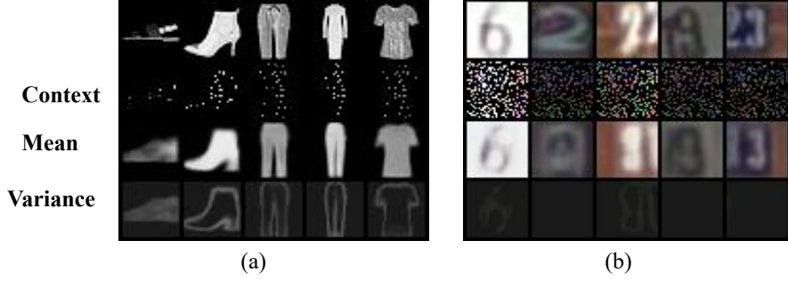
Figure 22: Examples of Completed Images using SI-NP. We randomly sample test images from FMNIST and SVHN datasets, and ground truth images are in the first row. The predictive means and variances of completed images are visualized in the third and fourth rows.
