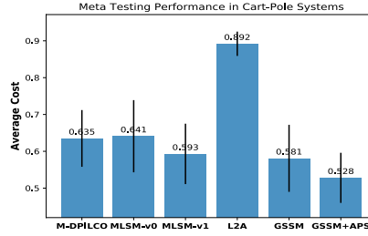
Figure 18: Meta Testing Performance. The average cost is negative of average rewards, and standard deviations are attached as error bars. For methods except GSSM+APS, additional time is required to perform gradient-based adaptation in policies.
