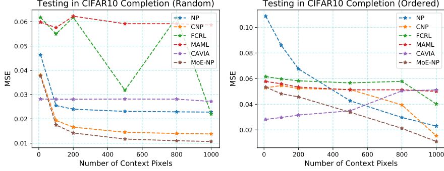
Figure 10: CIFAR10 Completion Performance with Various Number of Context Pixels. The numbers of context points used in prediction are 10, 100, 200, 500, 800, 1000. The left figure is with random context pixels while the right one is with the ordered context pixels.
