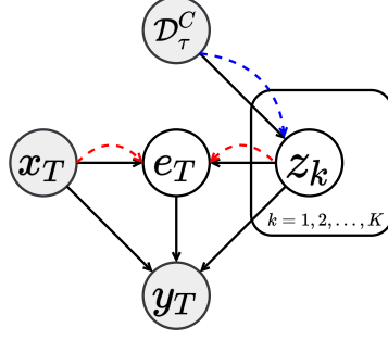
Figure 26: Computational Diagram in Meta Reinforcement Learning. This is in an information bottleneck form (Rakelly et al., 2019; Gondal et al., 2021). The variational posteriors are p_{\phi,k} = q_{\phi_{1,k}}(z|\mathcal{D}_\tau^C) and q_{\phi_2} = q_{\phi_{1,k}}(e|s, z_{1:K}) . As for the variational prior, we use the same strategy as that in (Rakelly et al., 2019). They are respectively the fixed normal p(z) = \mathcal{N}(0, I) and the categorical p(e) = \text{Cat}(e; K, [\frac{1}{K}, \frac{1}{K}, \dots, \frac{1}{K}]) .
