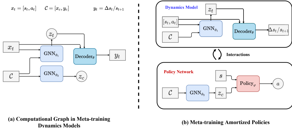
Figure 36: Computational Graphs of GSSM in Meta-training Processes. Note that amortized policy search is used here. On the Left side of the Figure: it describes the connections of variables in neural networks for meta dynamics models. On the Right side of the Figure: it illustrates the process in meta model-based policy search (Note that the reparameterization trick is used here and sampled latent variables z_t and z_c are deterministic, denoted by squares).
