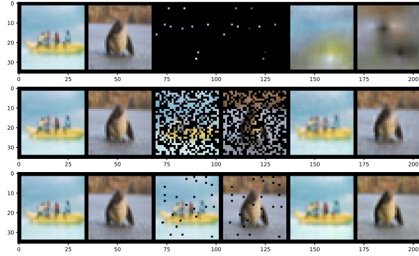
Figure 11: Image Completion Visualization using MoE-NPs. From top to bottom: the number of random context pixels is 10, 500, and 1000. From left to right (every two) are original, masked, and reconstructed images.
