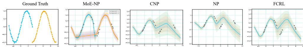
Figure 8: The Ground Truth and Predictive Distributions of Curves using NP related Models. The gray dots around curves are the context points. The shaded regions correspond to 3\times standard deviations. In MoE-NPs, two components of the sampled mixture curve in blue and orange can be identified via assignment latent variables with more than 85% accuracy.
