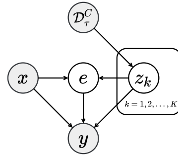
Figure 6: Generative Process of MoE-NPs. Here \mathcal{D}_\tau^C refers to dataset of context points in the paper. \{z_k\}_{k=1}^K are a set of expert latent variables and e is an assignment latent variable. Observed variables are grey in circles with latent variables white.
