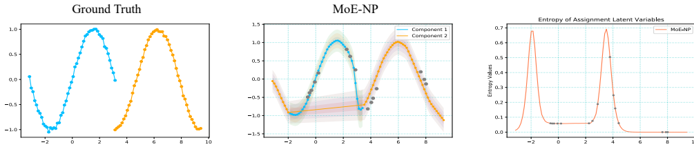
Figure 9: Entropy of Assignment Latent Variables in MoE-NPs. From left to right are respectively the sampled ground truth function, MoE-NP fitting results and the entropy value of discrete latent variable for each data point \mathbb{H}[p_{\phi_{2,2}}(e|z_{1:K}, x_i)] .
