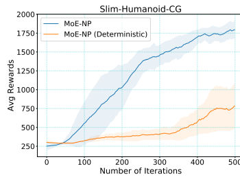
Figure 15: Ablation Performance in S-Humanoid-CG. Learning curves display tested average returns with variances in 4 runs.
