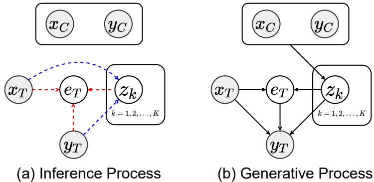
Figure 25: Computational Diagram in Few-shot Supervised Learning. Blue dotted lines are for expert latent variables, while red dotted lines are for assignment latent variables in inference.
