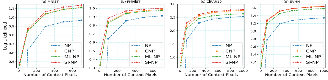
Figure 23: Asymptotic Performance in Image Completion. We meta test pixel average log-likelihoods with varying number of context points in image datasets. Context points are randomly selected for each image in testing processes. For MNIST/FMNIST datasets, the numbers of context pixels in testing are \{10, 100, 300, 500, 700\} . For CIFAR10/SVHN datasets, the numbers of context pixels in testing are \{10, 100, 300, 500, 800, 1000\} .
