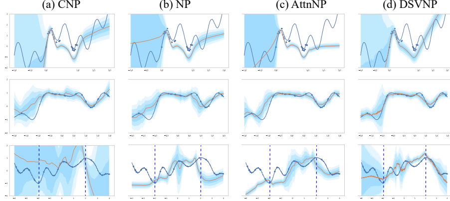
Figure 3: Function Prediction in Interpolation and Extrapolation. Blue curves are ground truth with dotted units as context points, and orange ones are predicted results. Rows from up to down indicate cases: single function with noise, interpolation, and extrapolation towards realizations from a stochastic process. The shadow regions are \pm 3 standard deviations from the mean.
