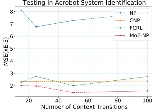
Figure 27: Asymptotic Performance in System Identification of NPs Family. The numbers of random transitions as the context are respectively {15, 25, 50, 100}.
