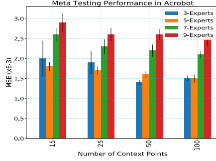
Figure 14: Predictive Performance of MoE-NPs in Acrobot Meta Testing Processes using Varying Numbers of Expert Latent Variables and Context Points. The scale for mean square errors together with standard deviations is E-3.
