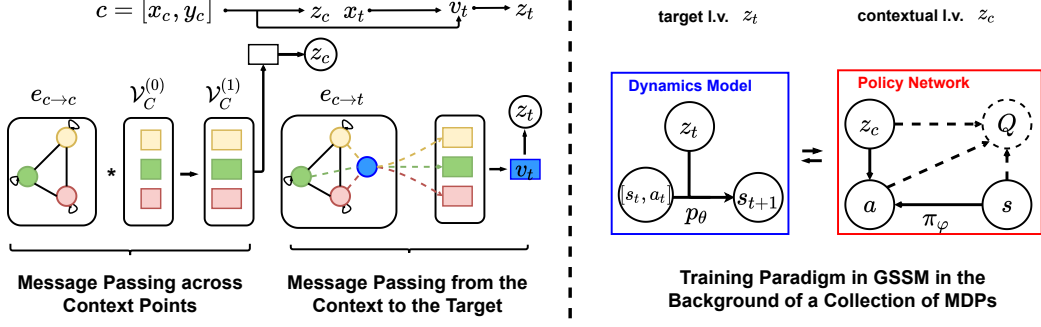
Figure 16: Graph Structured Surrogate Models. On the Left : The colored \square denotes a node feature vector in our fully connected graphs with nodes \bigcirc , and lines between \bigcirc record pairwise similarities \text{sim} . \mathcal{V}_C^{(0)} denotes the initial feature matrix of all context nodes. Information Flows in Dynamics Models from the left to the right describe the Message Passing between context points c (Edges in solid lines e_{c \rightarrow c} ) and to the target point t (Edges in dashed lines e_{c \rightarrow t} ) to obtain the transformed node feature matrix \mathcal{V}_C^{(1)} . On the Right : In amortized policy search, latent variables participate in both approximate Dynamics Models and Policy Networks (Dashed elements are involved in the module when using Actor-Critic frameworks and Double arrows mean interactions to learn amortized policies).
