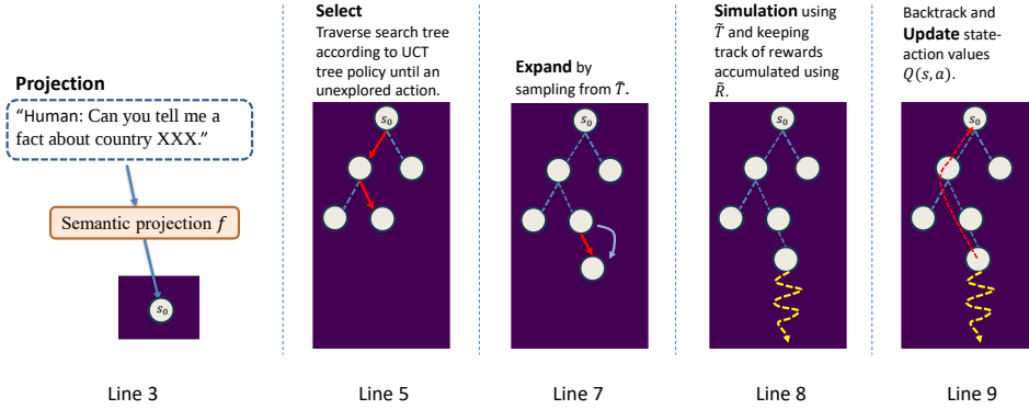
Figure 7: Visualization of SCOPE (Algorithm 1), which performs MCTS in semantic space with the help of semantic embedding function f , \tilde{T} and \tilde{R} (Sections 4.2 and 4.3).
