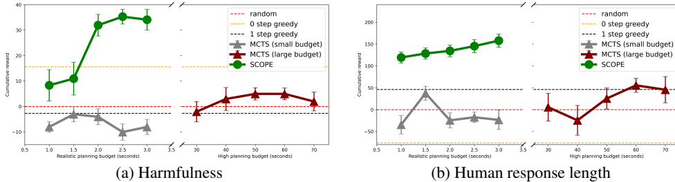
Figure 4: Comparison of SCOPE with larger planning budget vanilla MCTS (higher is better).
