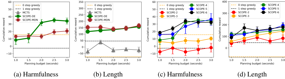
Figure 11: (a) and (b): Ablation study on how transition model choice affects SCOPE’s performance. SCOPE-DE uses deep ensembles (Lepikhin et al., 2021) while SCOPE-MDN uses MDNs (Bishop, 1994). (c) and (d): Ablation study on how search depth affect SCOPE’s performance.
