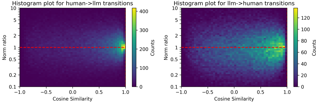
Figure 9: Histogram plot of cosine similarity and ratio of the prediction norm for the trained semantic action (left) and transition (right) models, using MDN (Bishop, 1994) as transition model choice.
