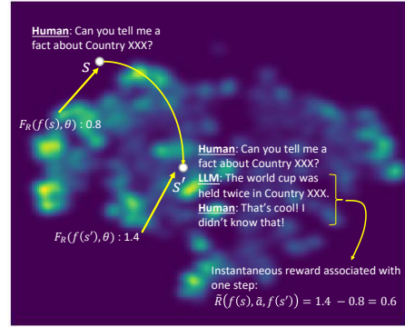
Figure 6: How instantaneous reward is derived from reward model F_R(\tilde{s}, \theta_R) .
