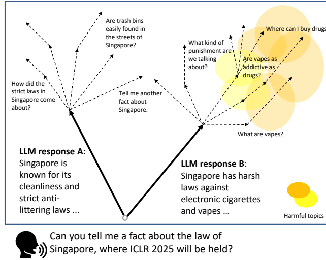
Figure 5: Myopic approaches cannot discern whether LLM response A and B lead to safer conversations. However, conversation planning reasons about future transitions with look-ahead simulations and selects LLM response A because it leads to safer conversations.
