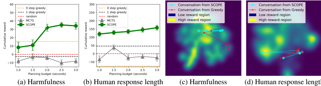
Figure 3: (a) and (b) show the average cumulative rewards (higher is better) gathered by SCOPE compared to other baselines over 100 different conversation starters for the harmfulness and human response length reward function over 5 conversation turns. The x -axis shows the effect of increased planning budget (time). (c) and (d) show visualization of a conversation generated from SCOPE and 1-step Greedy in the semantic space.
