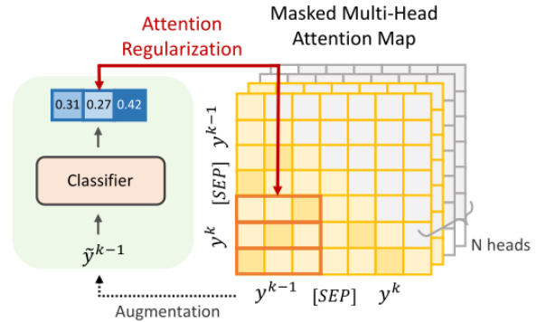
Figure 1: Instance-level context attention regularization mechanism. We obtain a continuous distribution of the target context by making perturbations ( \hat{y}^{k-1} ) to the target context y^{k-1} . We then regularize two attention heads of the top decoder layer.
