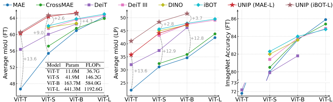
Figure 2: The performance of pre-trained models across various methods and sizes. Left : The average fine-tuning (FT) performance on three infrared semantic segmentation datasets, along with the associated computational cost. Middle : The average linear probing (LP) performance on three infrared datasets. Right : The fine-tuning performance on ImageNet (Deng et al., 2009). The gray dotted lines and corresponding values highlight the performance gains of UNIP over other methods. Detailed results for each dataset are presented in Tab. 11.
