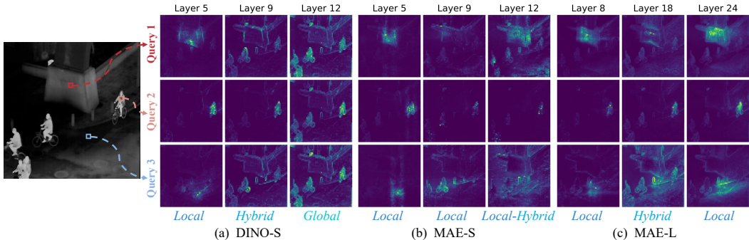
Figure 3: Attention maps for different query tokens in three representative layers. Each query token’s attention map corresponds to a row in the attention matrix, averaged over different heads.
