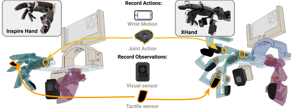
Figure 2: Exoskeleton Design. The optimized exoskeleton design shares the same joint-to-fingertip position mapping as the target robot hand while maintaining the wearability. The exoskeleton utilizes the encoder to precisely capture the joint action and 150° DFOV camera to record the information-rich visual observation. An iPhone is rigidly mounted to track the wrist pose through the ARKit.
