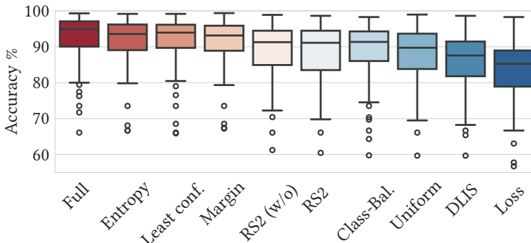
Fig. 8. Currently trained composite model accuracies for full data training and 50 % data selection on YEARBOOK.
