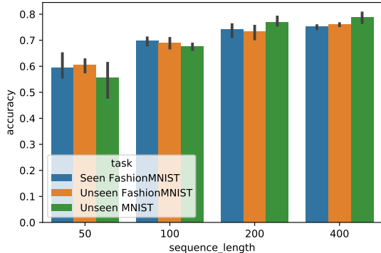
Figure 11: Increasing the sequence length during meta-training and meta-testing improves the predictive performance of the final query in the sequence. Error bars indicate 95% confidence intervals.
