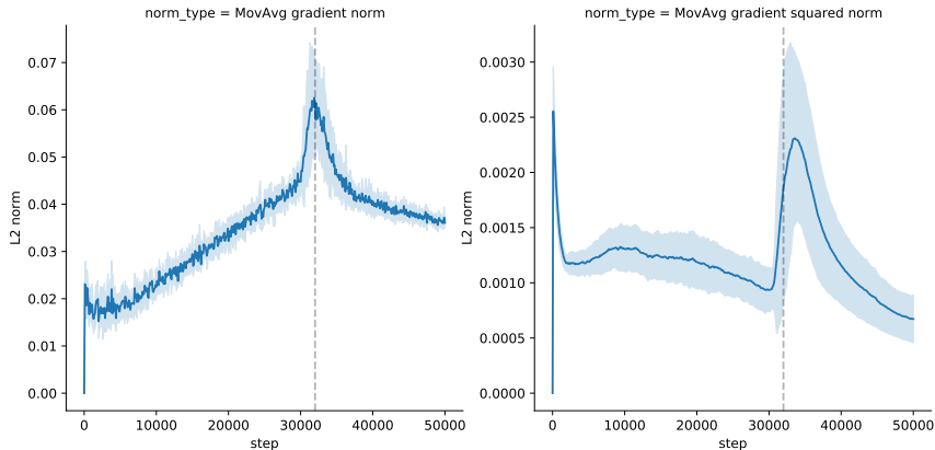
Figure 12: L2-norms of the gradient and squared gradient exponential moving average in Adam. The dashed line corresponds to the loss drop at the end of the loss plateau.
