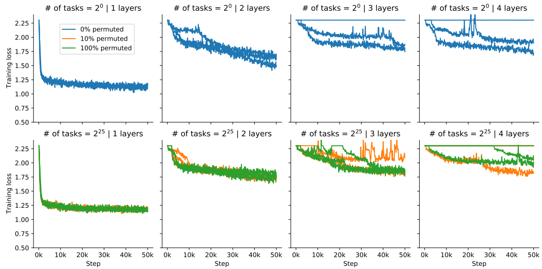
Figure 18: Loss plateaus and slow convergence with deeper variants of VSML.
