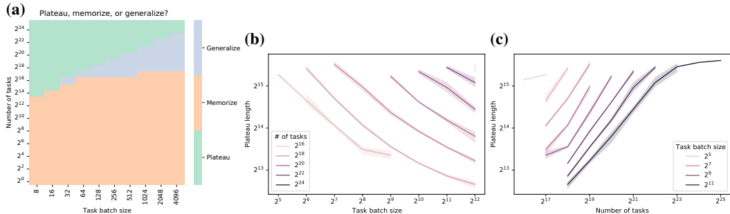
Figure 7: Whether GPICL memorizes, generalizes, or remains trapped on a meta-loss plateau depends on the number of meta-training tasks, and the meta-training batch size. (a) A phase diagram showing GPICL’s behavior at the end of meta-training (50k steps). Solutions either memorize, generalize and learn, or remain in the loss plateau. With additional training steps, configurations in the plateau might eventually transition to memorization or generalization. Generalization only occurs with large enough batch sizes and sufficient, but not too many, tasks. (b) This behavior is explained by the plateau length decreasing with the increasing batch sizes (reducing the noise contribution), and (c) increasing with larger numbers of tasks.
