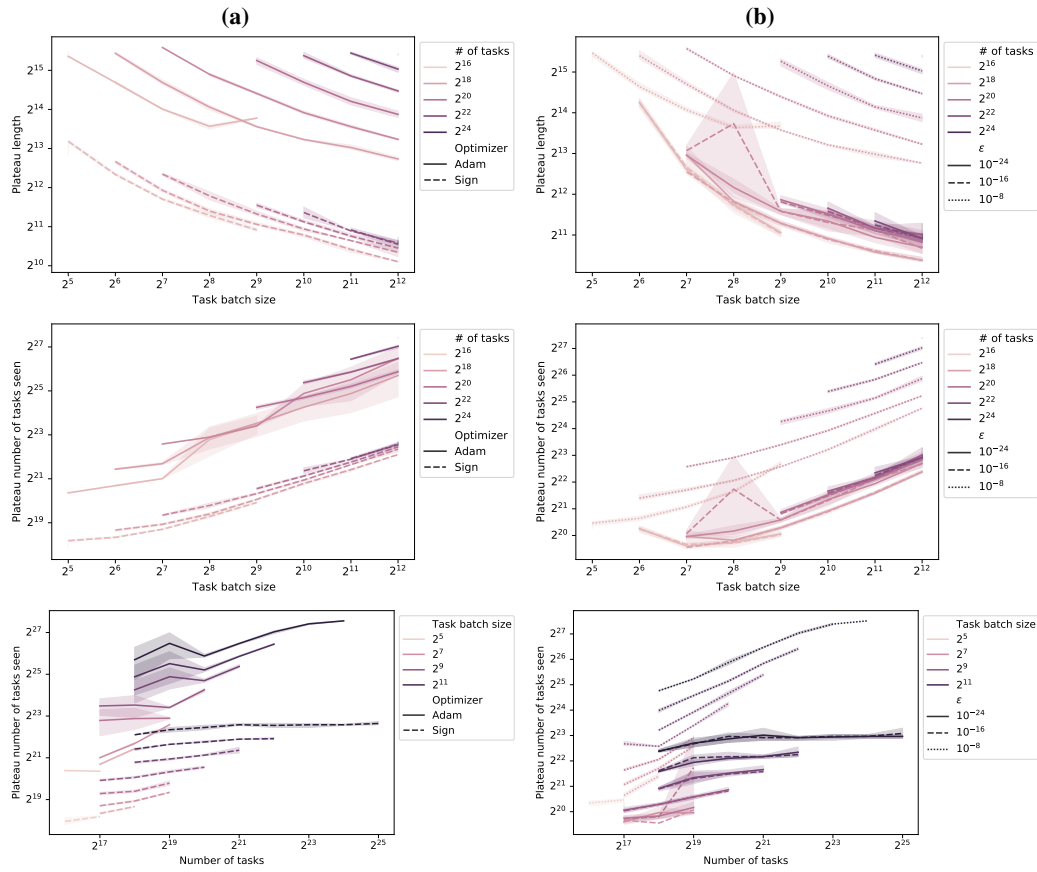
Figure 16: (a) When replacing Adam with a sign normalization of the gradient or (b) reducing \epsilon the plateau length is significantly shorter.
