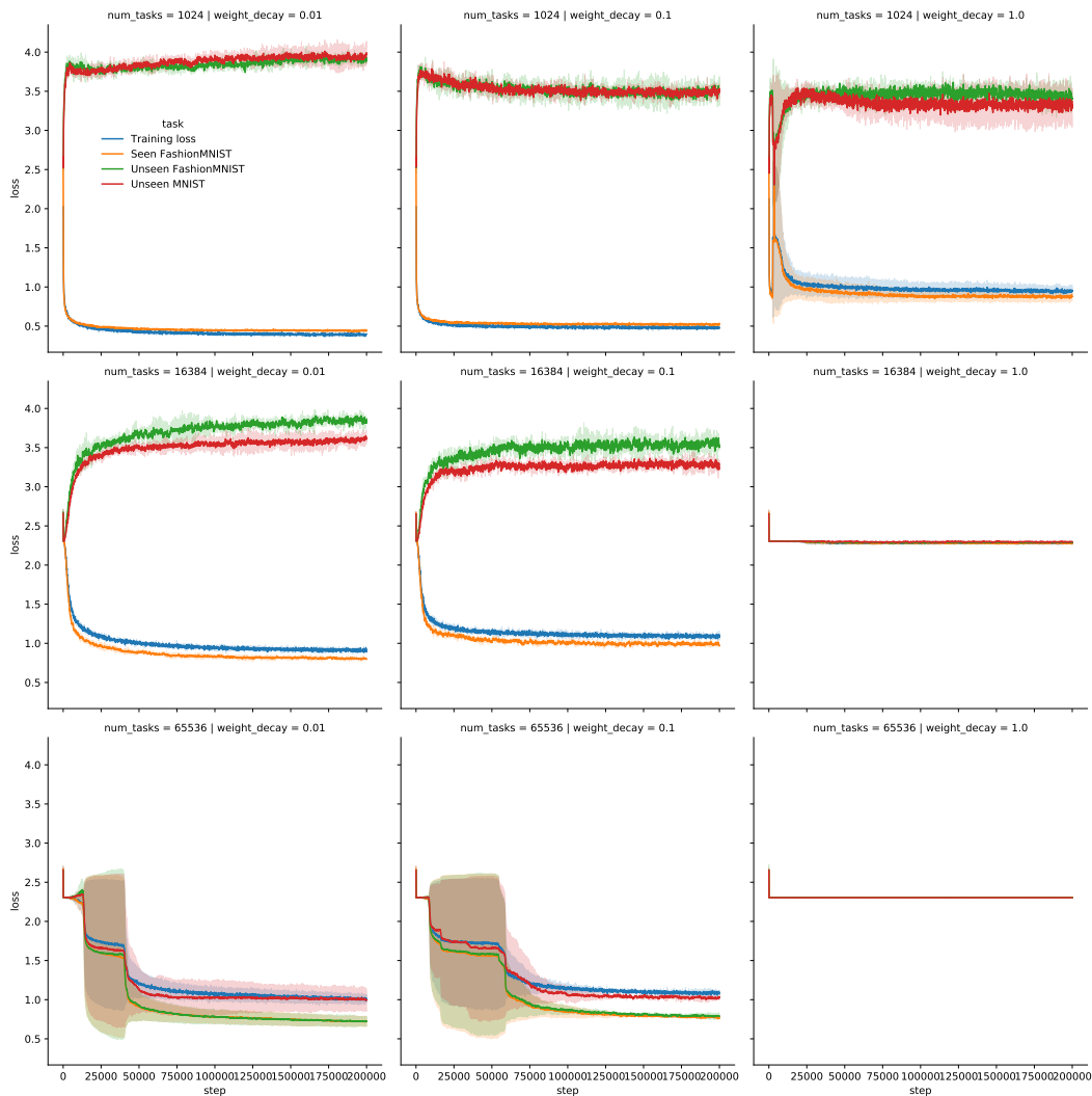
Figure 17: We investigate whether grokking as defined in Power et al. (2022) can be produced when we observe memorization on a smaller numbers of tasks. This would correspond to the test loss decreasing long after the training loss has converged. We have not been able to elicit this behavior when looking at different numbers of tasks and weight decay coefficients.
