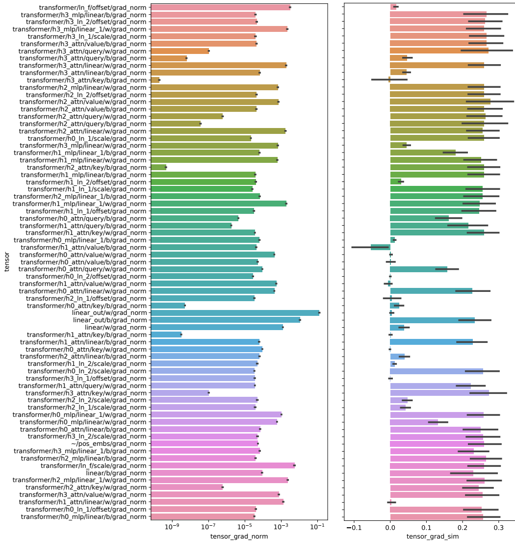
Figure 14: Gradient L2 norms (left) and gradient cosine similarity for consecutive optimization steps (right) for different parameter tensors. The last (output) layer has the largest gradients. Most other gradients are small.
