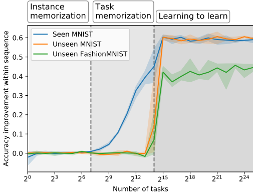
Figure 4: Transformers exhibit three different phases in terms of meta-learned behavior. (1) When training on a small number of tasks, specific instances are memorized. (2) Tasks are memorized, which is evident as a within-sequence increase of performance. (3) When training across many tasks, we discover a learning algorithm that generalizes to unseen tasks and unseen datasets.
