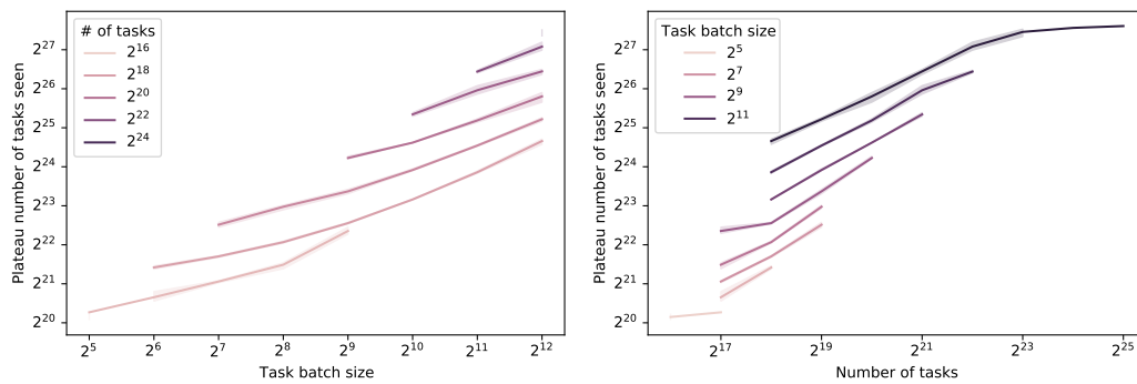
Figure 15: Instead of plotting the loss plateau length in terms of optimization steps, we look at the total number of tasks seen within the plateau as a function of the task batch size and the number of tasks in the training distribution. An increase in the task batch size leads to more tasks to be processed to leave the plateau.
