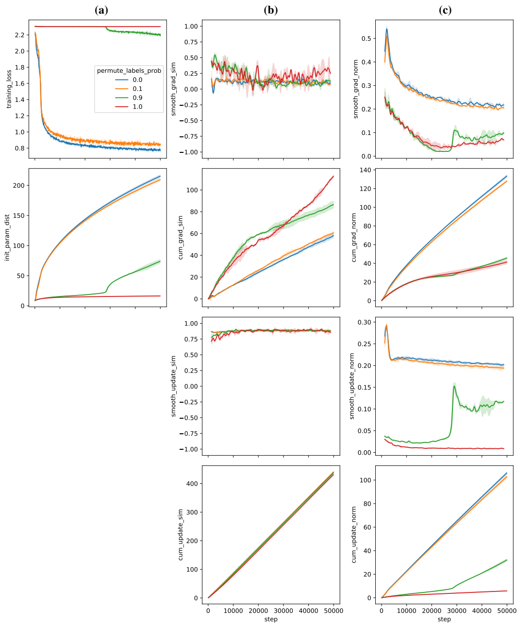
Figure 13: Gradient and Adam update statistics for differently biased data distributions. (a) Plateaus in the loss are influenced by the bias in the data distribution. Plateaus result in moving away slowly from the parameter initialization. (b) The cosine similarity of both gradients and updates in consecutive steps is only marginally different with or without a loss plateau. (c) While the gradient norm is about half as big when a plateau exists, the updates are going towards zero.
