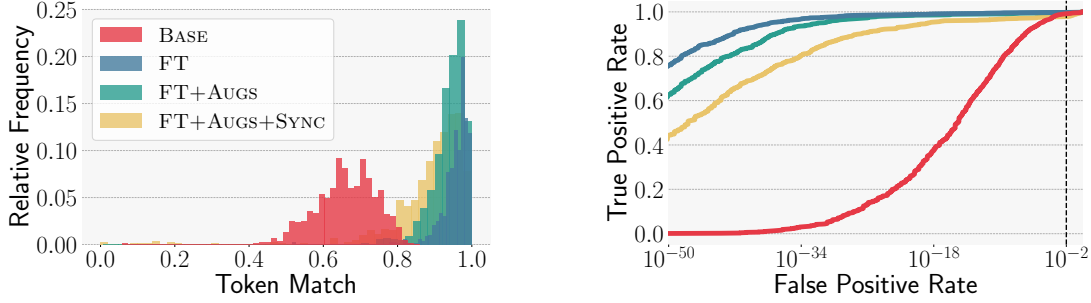
Figure 5: Left: Finetuning improves token match (Eq. (3)) between original and re-tokenized image tokens. Right: All variants achieve TPR \approx 1 at FPR of 1%. Finetuning further boosts detection in low-FPR settings.
