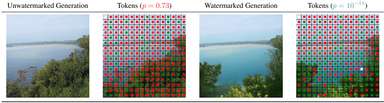
Figure 2: Example of our watermark on an autoregressively generated image. We generate the upper half of the image without the watermark. We then complete the bottom half in the same way (left) or with the watermark (right). The overlay indicates generated image tokens detected as green (■), red (■), or ignored as a duplicate (□). The watermark only alters semantics and could be detected even when applied only partially as in this case.
