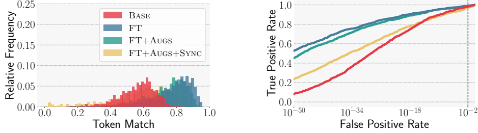
Figure 13: Token match and watermark power results for CHAMELEON. Left: Finetuning improves token match (Eq. (3)) between original and re-tokenized image tokens. Right: All variants achieve TPR \approx 1 at FPR of 1%. Finetuning further boosts detection in low-FPR settings.
