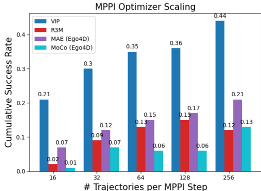
Figure 15: VIP vs. Alternative Pre-Training Algorithms on Ego4D.
