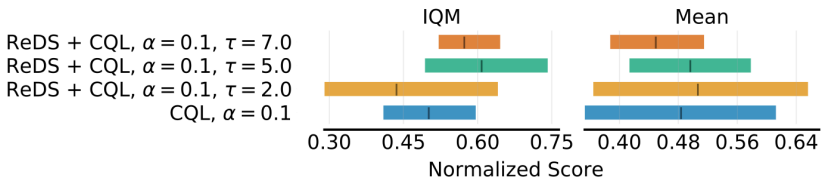
Figure 12: Sensitivity of CQL (ReDS) to the temperature hyperparameter \tau in Equation 9 evaluated on the Atari game experiments with 5 policies. Observe that an intermediate value of temperature \tau = 5.0 works best
