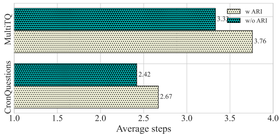
Figure 5: Comparison of average reasoning steps of ARI in MULTITQ.
