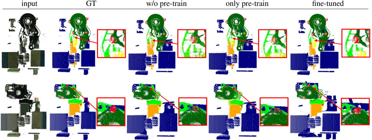
Figure 4: Segmentation result visualization on real-world test data. Without pre-train means the network is trained on real-world data directly. Only pre-train means the network is trained only on synthetic dataset and directly used for the testing on real-world data. Fine-tuned means the network is both pre-trained and fine-tuned.
