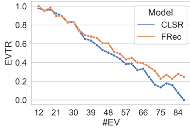
Figure 8: Online EVTR comparison between CLSR and FRec.
