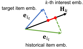
Figure 3: Illustration of the calculation of interest-aware similarity, represented by the length of the red line.
