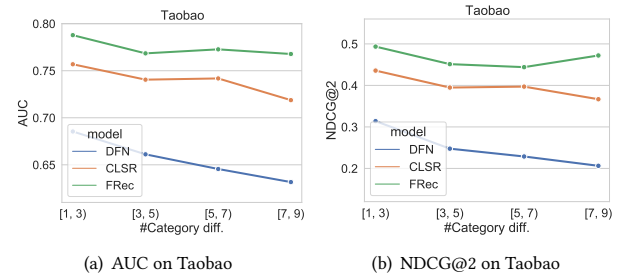
Figure 7: Performance of instance groups with different m .
