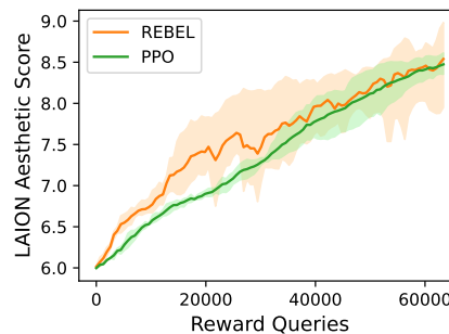
Figure 4: Learning curves as a function of reward queries to the LAION aesthetic predictor. The colored areas represent 95% CIs.
