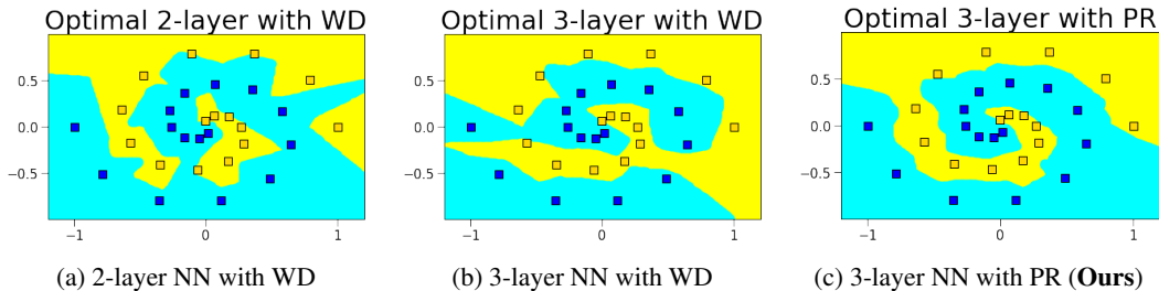
Figure 1: Decision boundaries of 2-layer and 3-layer ReLU networks that are globally optimized with weight decay (WD) and path regularization (PR). Here, our convex training approach in (c) successfully learns the underlying spiral pattern for each class while the previously studied convex models in (a) and (b) fail (see Appendix A.1 for details).
