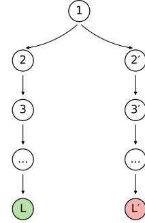
Figure 2: Toy DAG.
