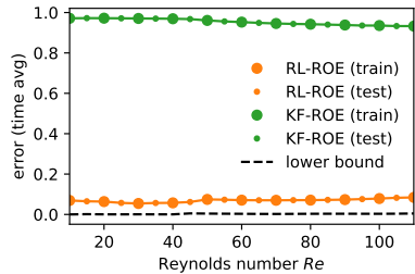
Figure 7: Navier-Stokes equations with p = 3 sensors. Time average of the normalized L_2 error versus Re . Values of Re present in Z_{\text{train}} shown by large circles.
