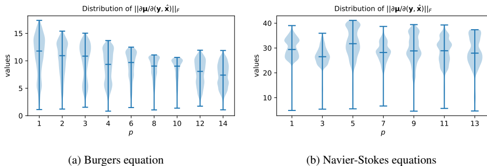
Figure 15: Nonlinearity of the trained policies obtained in the (a) Burgers and (b) Navier-Stokes examples for various p . Distribution of the Frobenius norm of the Jacobian of the trained mean policy \mu_{\theta^*} , sampled along solution trajectories of the RL-ROE.
