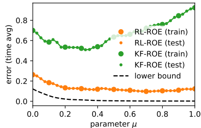
Figure 3: Burgers equation with p = 4 sensors. Time average of the normalized L_2 error versus \mu . Values of \mu present in \mathcal{Z}_{\text{train}} shown by large circles.
