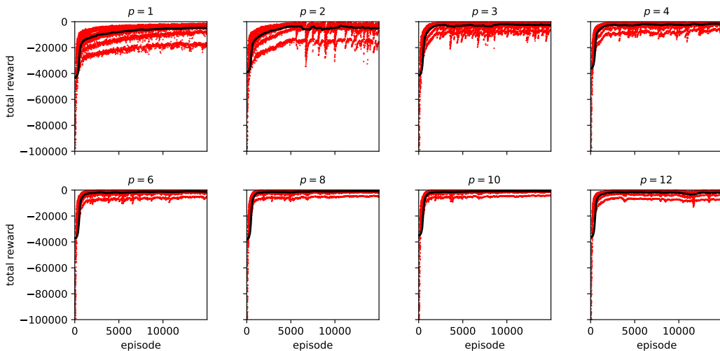
(a) Burgers
