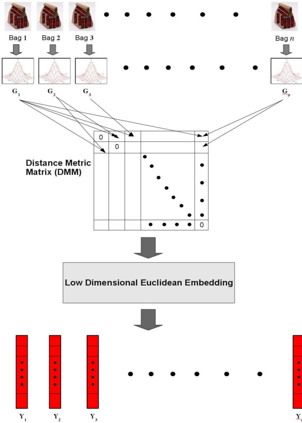
Figure 1: Outline of the proposed framework for unifying the representation of sets of vectors. In the first step, each bag of features , or set of vectors (SOV) is modelled as a Gaussian distribution. In the second step, a dissimilarity measure for the difference between Gaussian densities is selected and used to fill a distance metric matrix (DMM) with the dissimilarity, or the distance between every pair of Gaussian distributions. Note that this matrix is symmetric with zero diagonal elements (or self distances). In the third step, Euclidean embedding, or classical MDS is used to collectively embed all SOVs in a low dimensional Euclidean space. The final result is that each bag i is represented by a single vector y_i .
