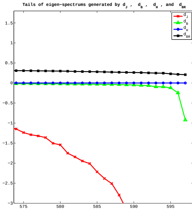
Figure 4: Tails of eigen-spectrums for the four similarity matrices shown in Figure (3). Note how the semi-metrics d_J and d_B yield negative eigenvalues, indicating that K_J and K_B are negative definite matrices and not PSD as required by Theorem 2.1.
