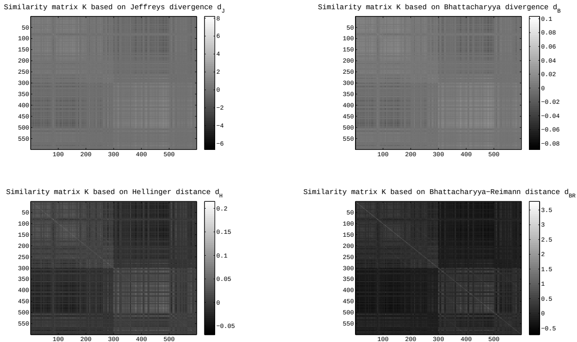
Figure 3: The four similarity matrices \mathbf{K}_J top left, \mathbf{K}_B top right, \mathbf{K}_H bottom left, and \mathbf{K}_{BR} bottom right. Note the clear block structure for \mathbf{K}_{BR} compared to other matrices.
