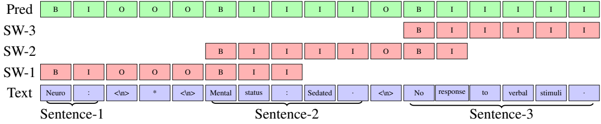
Figure 1: Sliding window algorithm for sentence segmentation. We segment the text using three sliding windows sequentially ( SW-1 , SW-2 , and SW-3 ). The final sentence segmentation tags are at the top ( Pred ) of the diagram.
