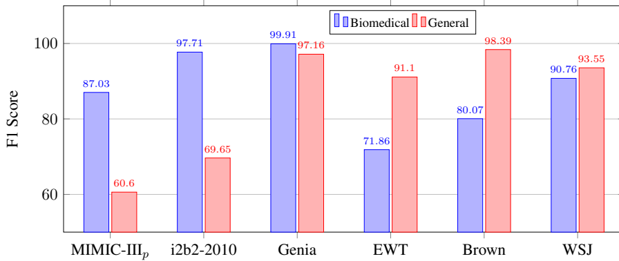
Figure 3: Cross-domain evaluation of our two Segmenter-Domain models.
