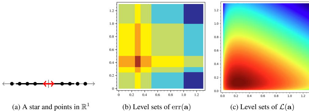
Figure 2: An example of a 1-dimensional dataset, perfectly classified by a star supported on a fan with n=2 rays, and the level sets of the two loss functions in parameter space \mathbb{R}_{>0}^2 . This example is explained in detail in Appendix A.2.
