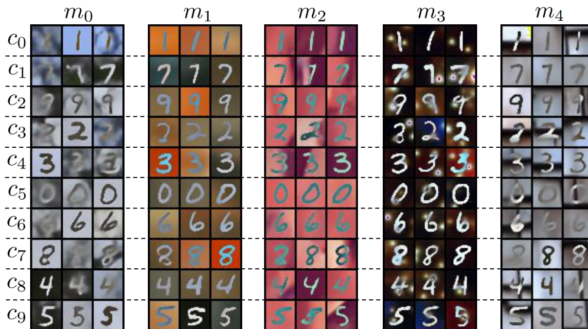
Figure 5: Generative qualitative examples of the clustering capabilities of CMVAE on PolyMNIST dataset. Each column corresponds to the generated samples of one of the five modalities, while each row reports three generation results for a different latent cluster.
