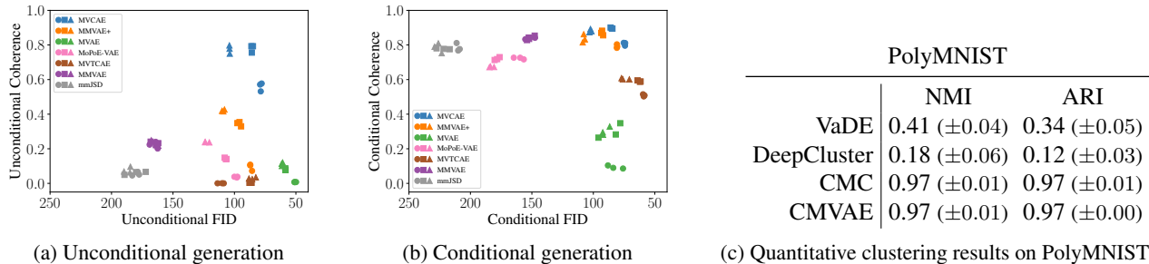
Figure 1 (a),(b): Generative performance comparison of CMVAE with multimodal VAEs on PolyMNIST. Three independent runs for each model, with different symbols denoting different values of the \beta hyperparameter. In both plots, generative coherence is measured on the y-axis (higher is better), while on the x-axis generative quality is assessed via the FID-score (lower is better). Therefore optimal performance is at the top-right corner of each plot. Table 1 (c): Quantitative clustering performance comparison on PolyMNIST.
