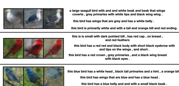
Figure 3: Qualitative results for CMVAE on the CUBICC dataset. For each row, three samples for both modalities are sampled from a different latent cluster.
