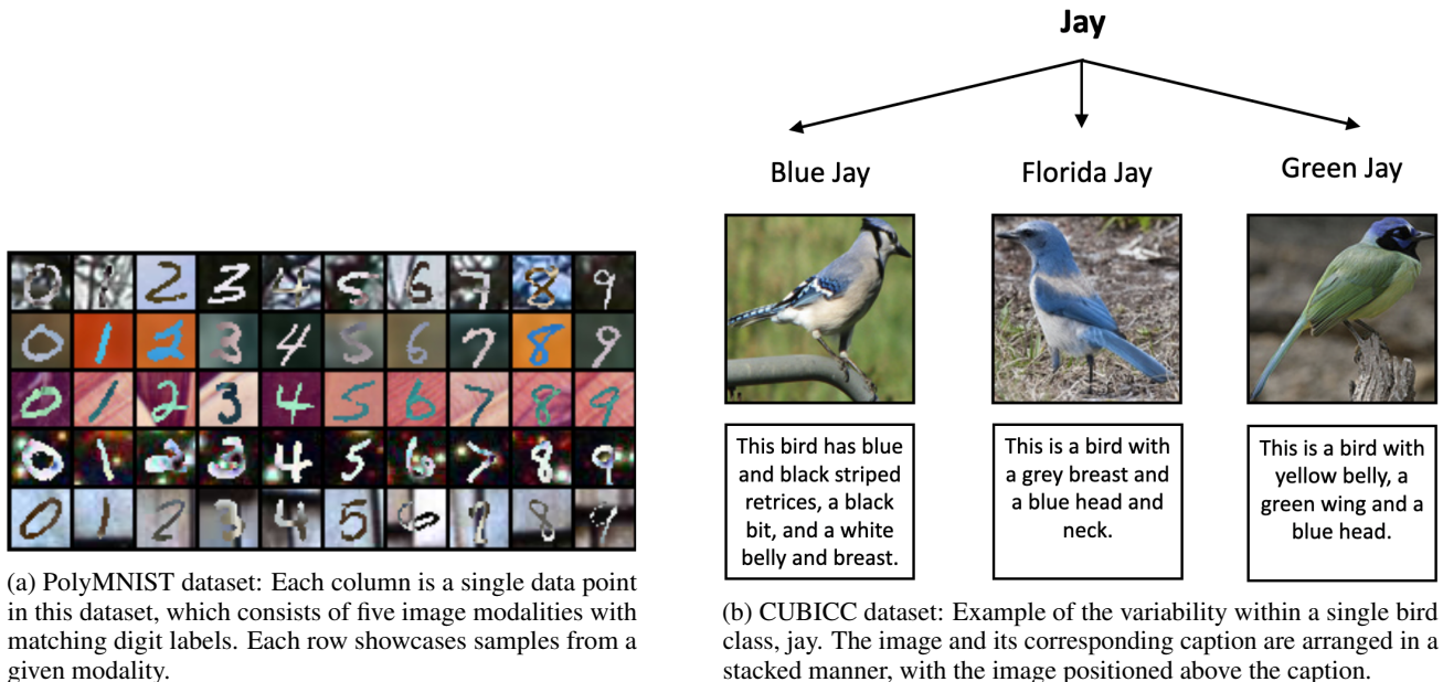
Figure 4: Illustrative samples for our considered experimental settings, PolyMNIST in (a) and CUBICC in (b).
