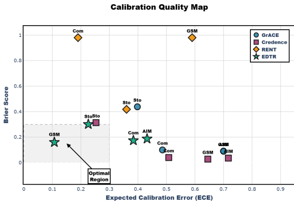
Figure 3: Calibration quality results comparing EDTR against other methods. Points located in the lowest left region are optimal results. Each point correlates one of 4 different datasets.
