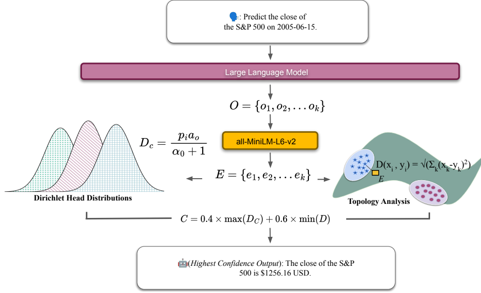
Figure 2: A sample prompt is put into an LLM and then enters an encoder model: all-MiniLM-L6-v2. Topology and Dirichlet Head combine to increase the confidence and produce the final output of the highest confidence.
