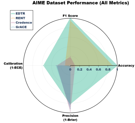
Figure 1: AIME performance results across four metrics for four methods including EDTR, RENT, Credence, and GrACE. The highest score for all metrics is desired.
