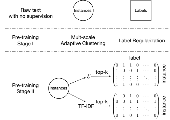
Figure 3: Framework of our pre-training procedure.
