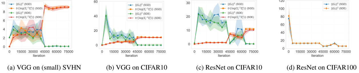
Figure 2: Gradient-related quantities of SGD or its discrete SDE approximation. In (d), since per-sample gradient is ill-defined when BatchNormalization is used, we do not track \text{tr} \left\{ \log \left( \Sigma_t^{-1} \Sigma_t^\mu \right) \right\} .
