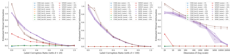
Figure 4: Mutual information estimation on Gaussian blobs.
