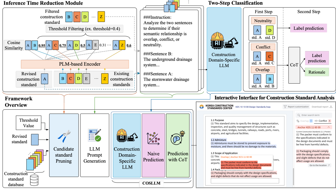
Figure 2: Overview of COSLLM and a real-time construction standards analysis framework. Our framework leverages an inference time reduction module to efficiently filter out irrelevant sentence pairs before LLM inference. It then performs effective classification of overlapping and conflicting sentences through a two-step classification process. Finally, the results are delivered to users via an interactive interface, which highlights overlap and conflict sentences, allows result viewing, and supports downloading for optimal usability.
