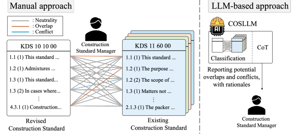
Figure 1: An overview of the manual and LLM-based approaches for analyzing overlapping and conflicting content in construction standards is provided. Using the proposed COSLLM, managers can review potential overlaps and conflicts identified by the LLM, along with detailed rationales, which significantly reduces manual effort.
