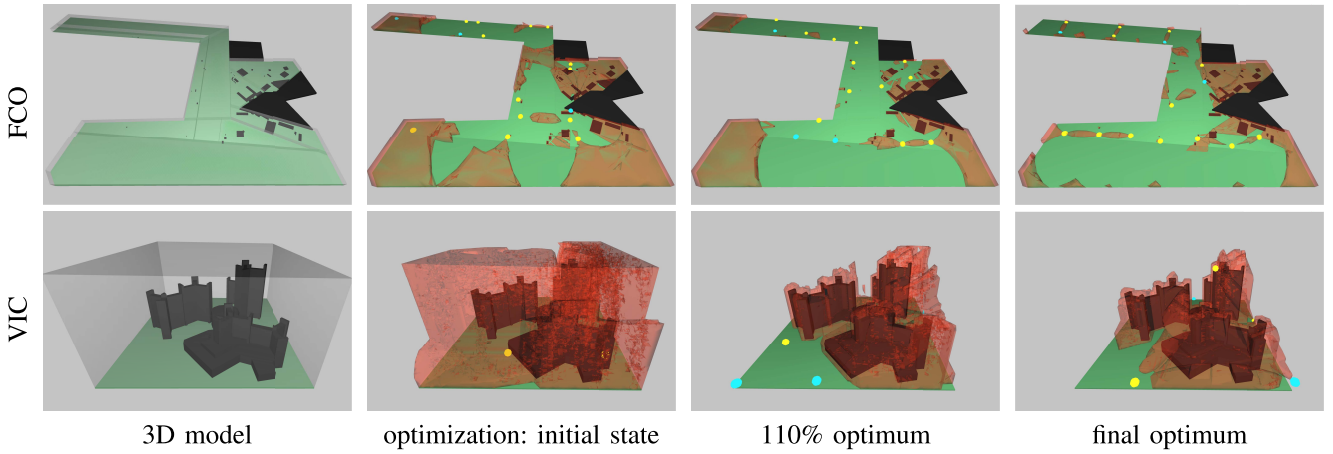
Fig. 6. 3-D models of our case studies and computation of optimal deployments at different states of search (green: RoI; red: uncovered region under no sensors faults).
